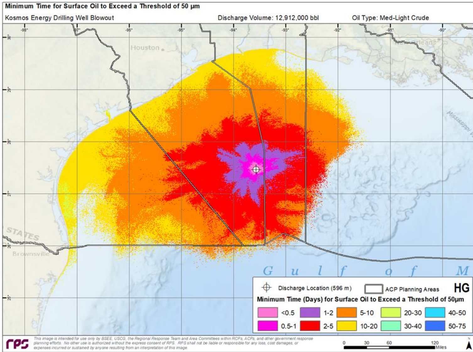
Figure 17. Minimum Travel Time for Surface Oil exposure greater than 50 \mu\text{m} .
