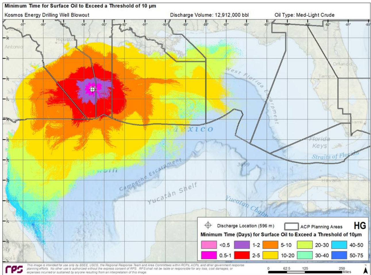
Figure 11. Minimum Travel Time for Oil on the Water Surface with Average Thickness greater than the Ecological Threshold of 10 \mu m.
