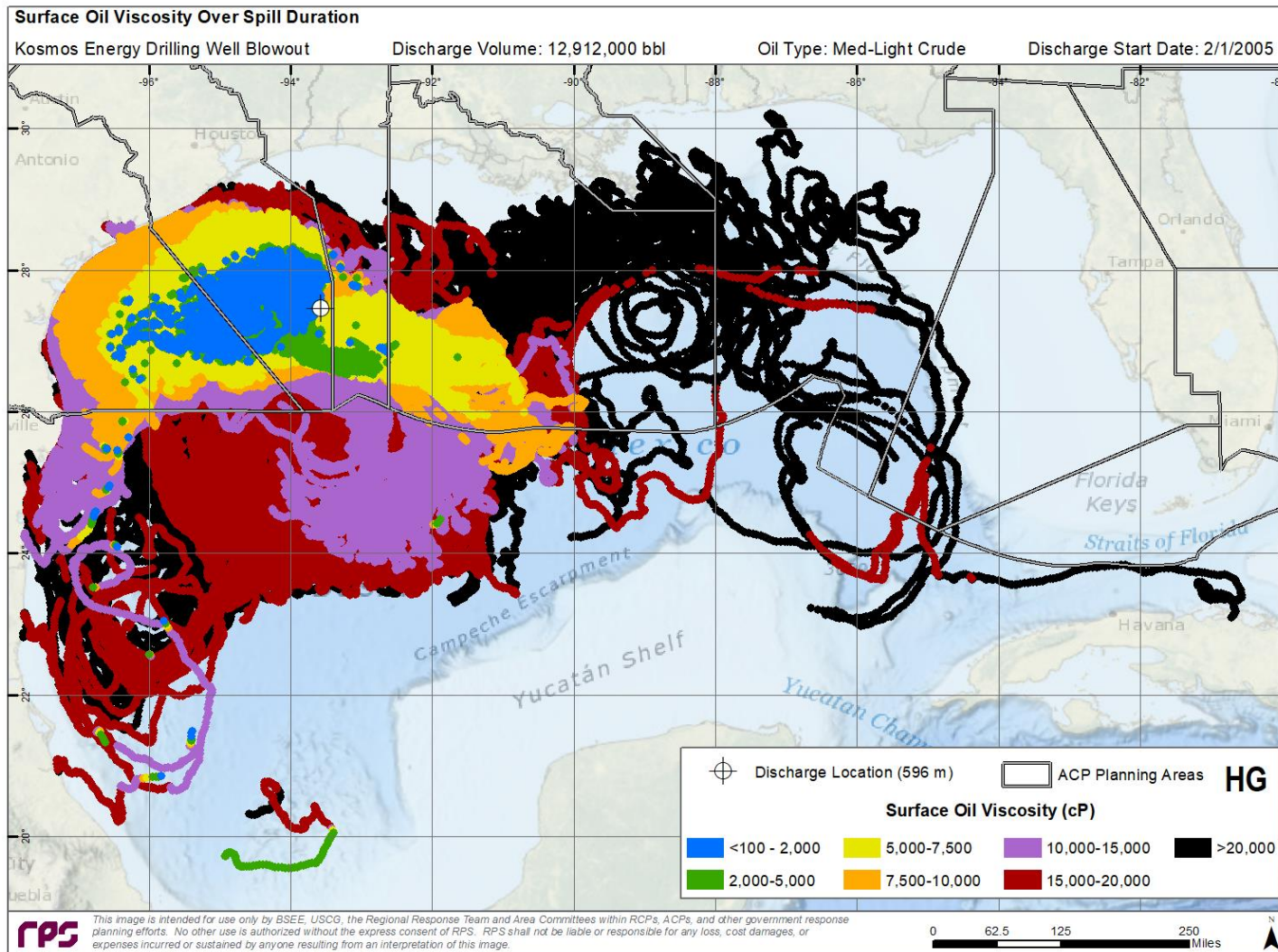
Figure 19. Cumulative footprint of exposure to surface floating oil greater than the minimum oil viscosity over a 75-day period for the worst case deterministic simulation. Viscosities greater than those mapped may be present at any location at any specific time in the simulation. This graphic provides a perspective of how oil viscosity may change as oil is transported away from the discharge site over time and what areas may be amenable to dispersant operations where enough quantities of oil are present.
