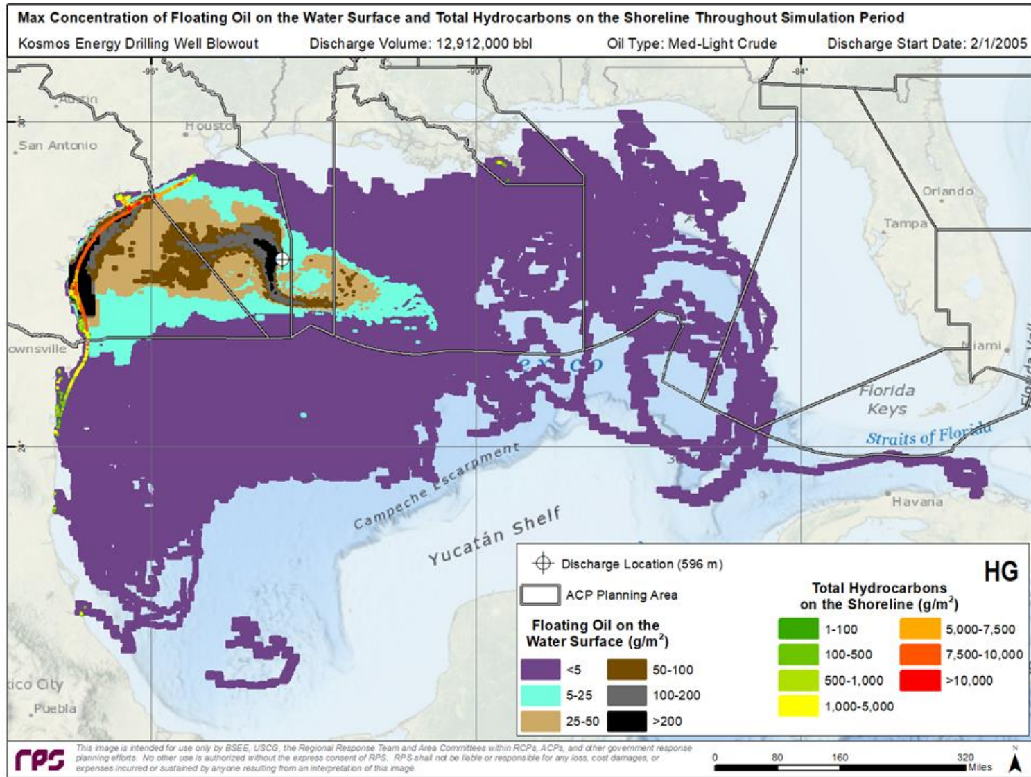
Figure 18. Cumulative Maximum Concentration of Floating Oil and Total Hydrocarbons on the Shoreline at any time during the worst case deterministic simulation.
