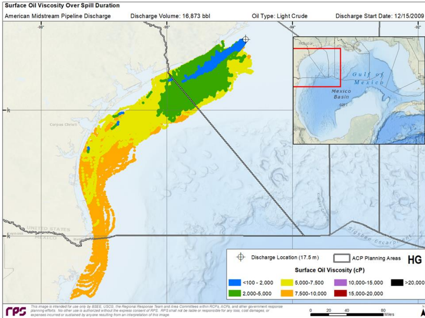
Figure 9. Cumulative footprint of exposure to surface floating oil greater than the minimum oil viscosity over a 45-day period for the worst case deterministic simulation. Viscosities greater than those mapped may be present at any location at any specific time in the simulation. This graphic provides a perspective of how oil viscosity may change as oil is transported away from the discharge site over time, and what areas may be amenable to dispersant operations where enough quantities of oil are present.
