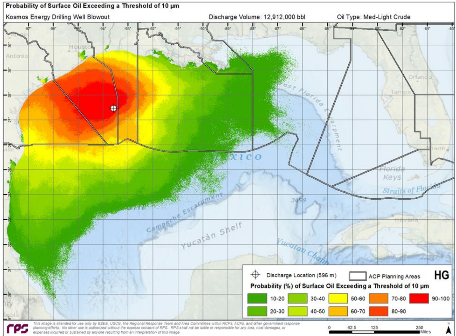
Figure 10. Probability Footprint for Oil on the Water Surface with Average Thickness greater than the Ecological Threshold of 10 \mu
