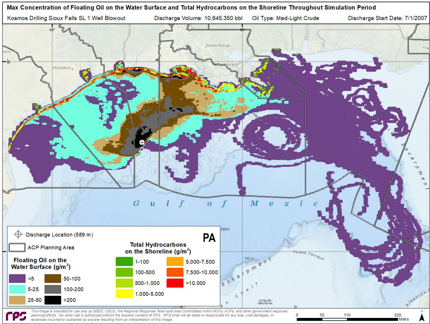
Figure 18. Cumulative Maximum Concentration of Floating Oil on the Water Surface and Total Hydrocarbons on the Shoreline at any time during the worst-case deterministic simulation.
