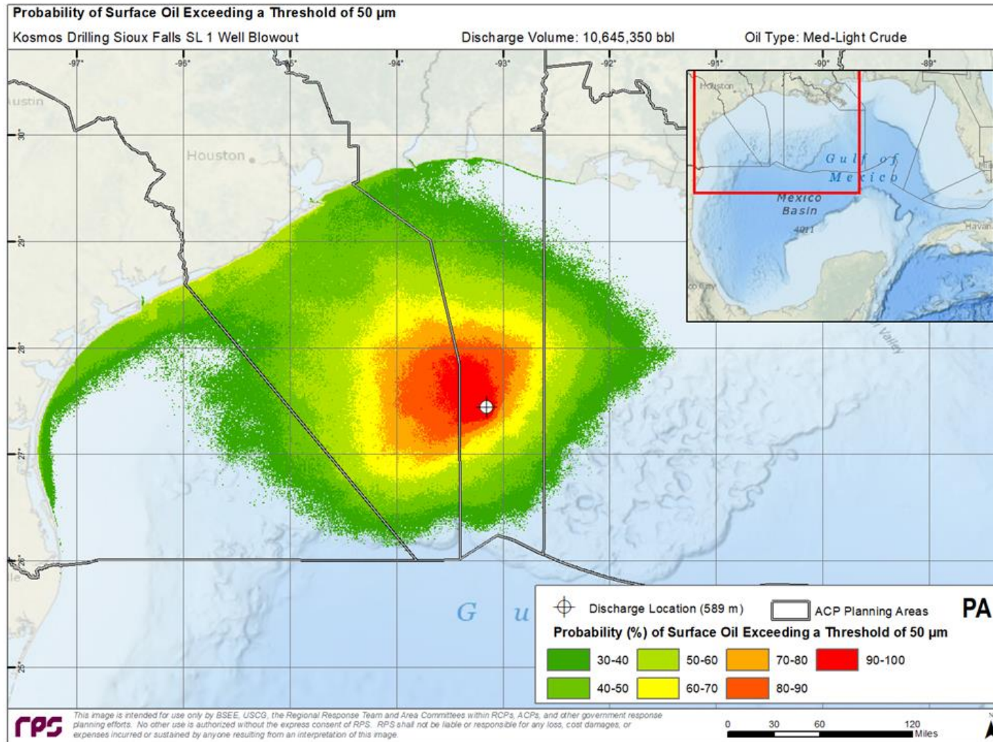
Figure 16. Probability Footprint for Surface Oil exposure greater than 50 µm. In this thickness range, oil will appear as a continuous to discontinuous patches of dark oil in quantities where high volume on-water mechanical recovery operations will be the most productive.
