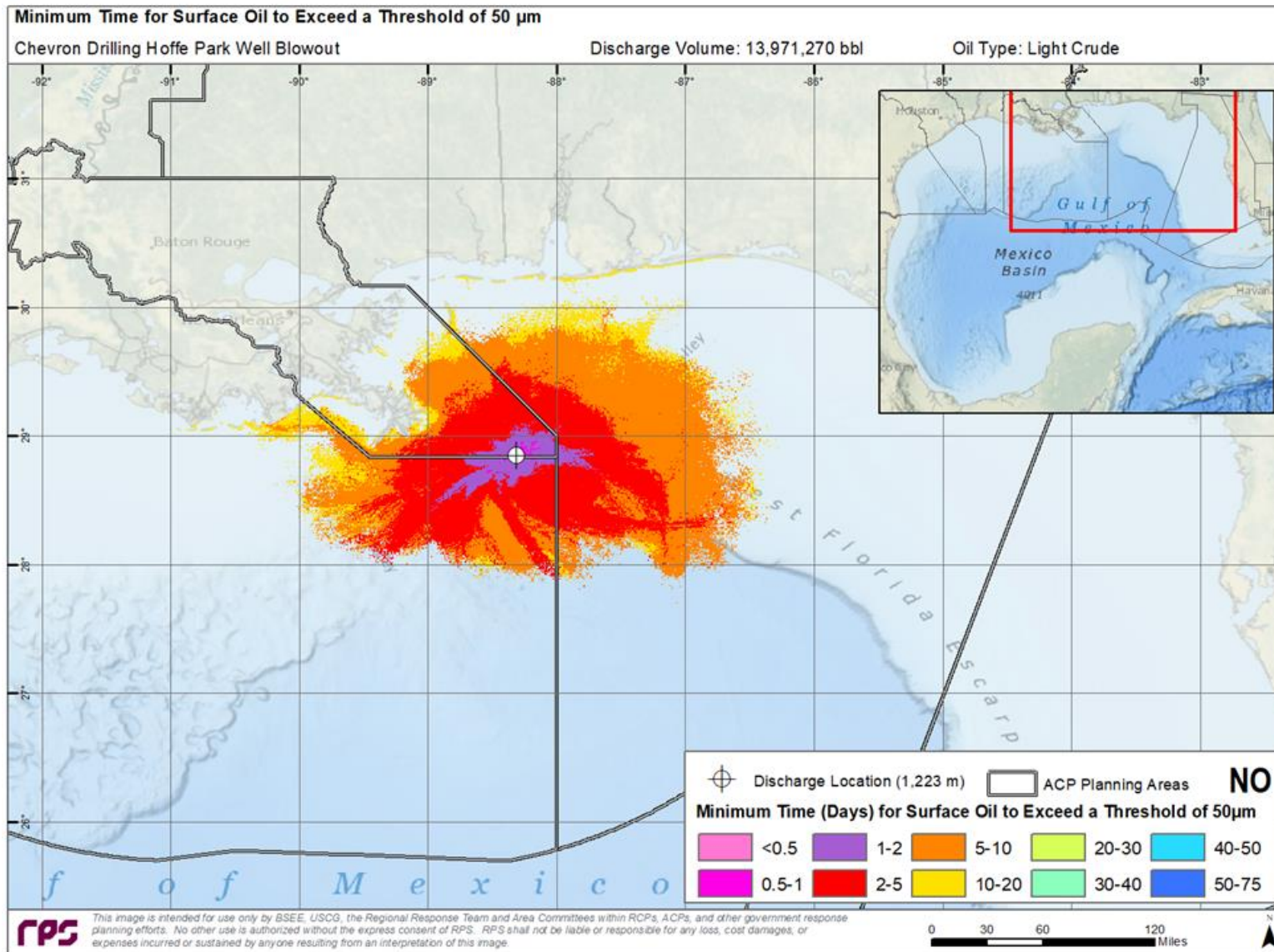
Figure 18. Minimum Travel Time for Surface Oil exposure greater than 50 \mu\text{m} .
