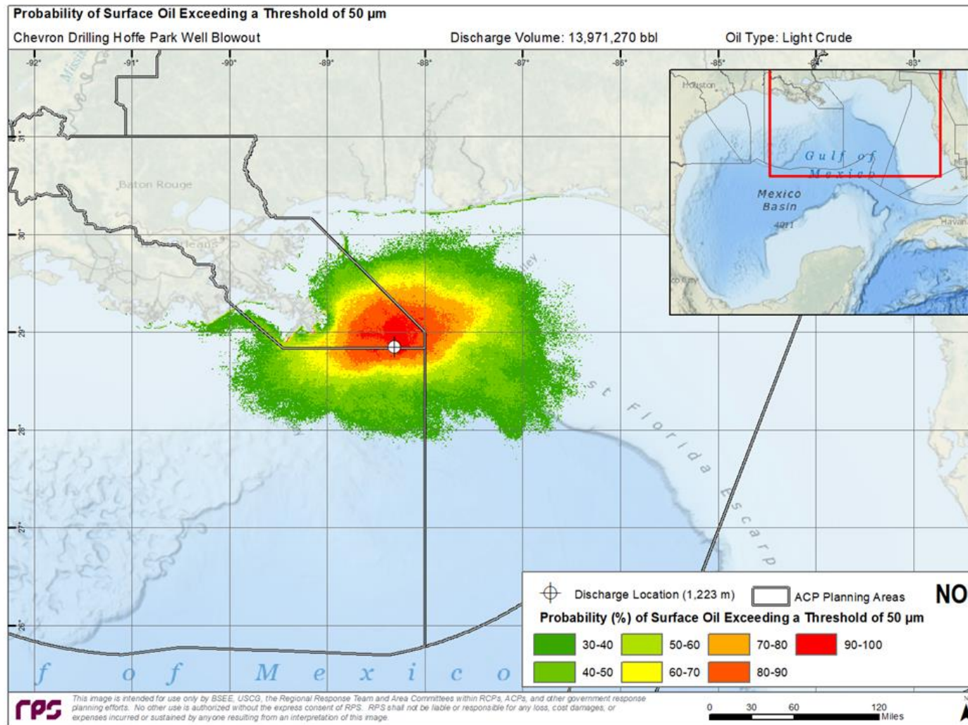
Figure 17. Probability Footprint for Surface Oil exposure greater than 50 \mu\text{m} . In this thickness range, oil will appear as a continuous to discontinuous patches of dark oil in quantities where high volume on-water mechanical recovery operations will be the most productive.
