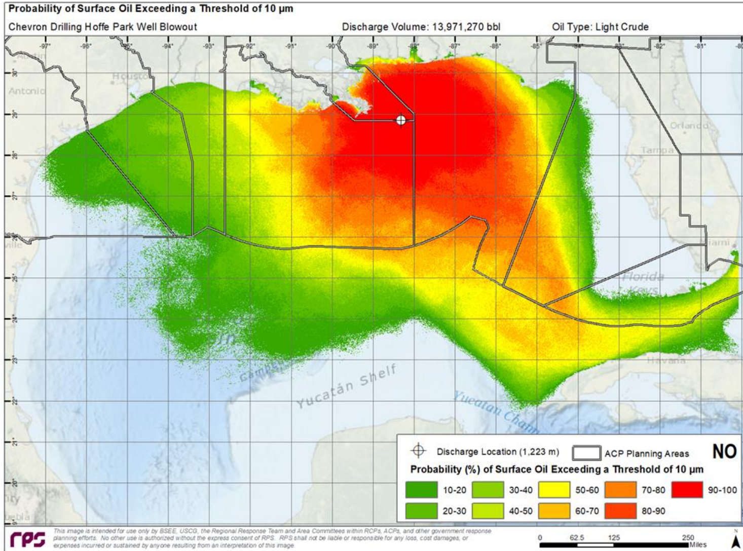
Figure 11. Probability Footprint for Oil on the Water Surface with Average Thickness greater than the Ecological Threshold of 10 µm.
