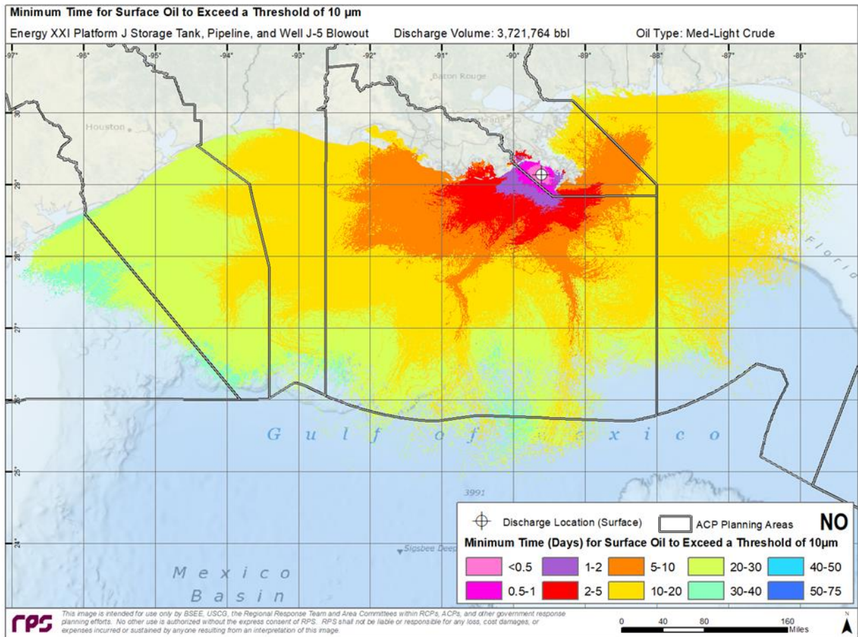
Figure 2. Minimum Time for Oil on the Water Surface with Average Thickness greater than the Ecological Threshold of 10 µm.
