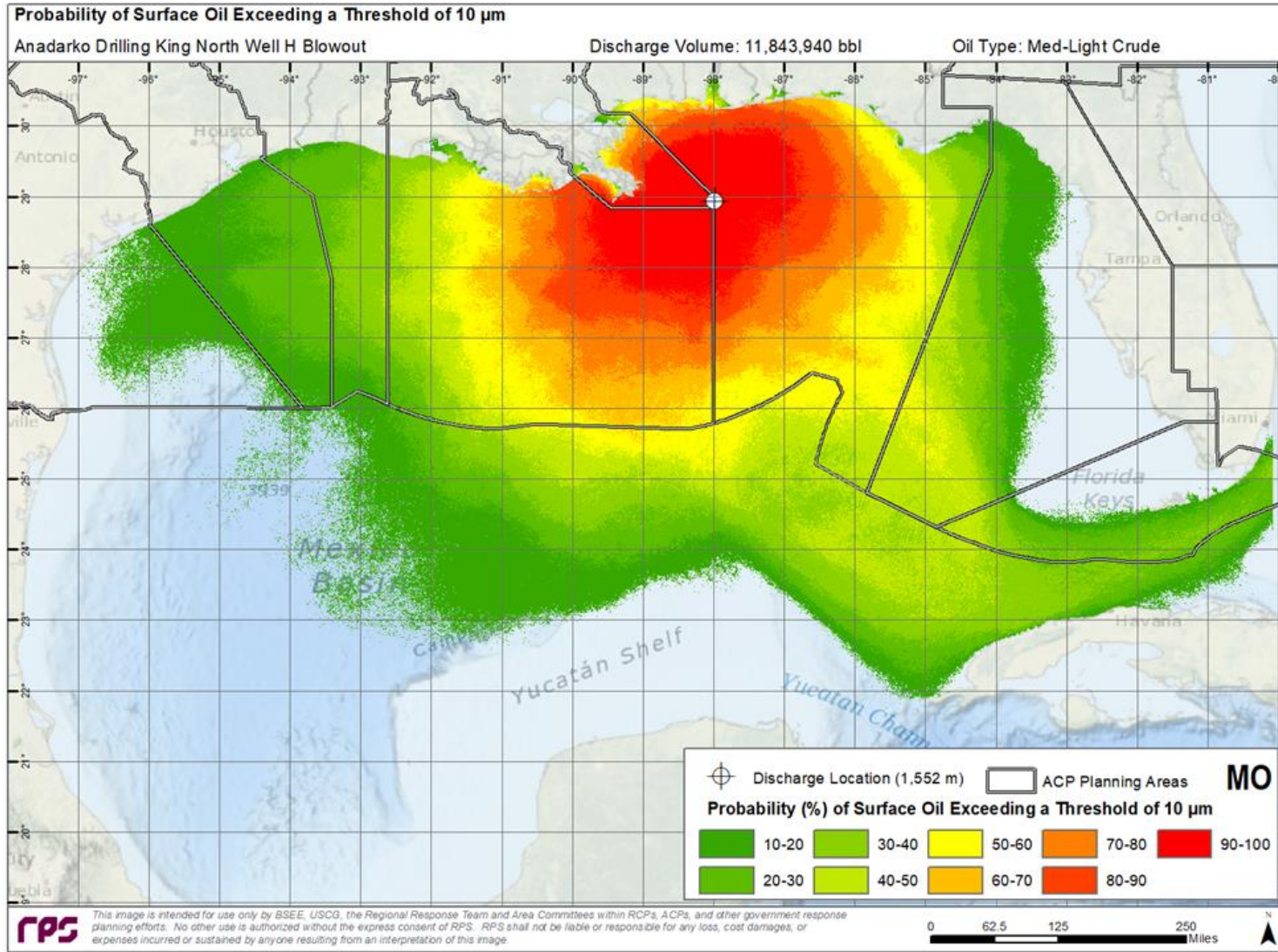
Figure 9. Probability Footprint for Oil on the Water Surface with Average Thickness greater than the Ecological Threshold of 10 \mu\text{m} .
