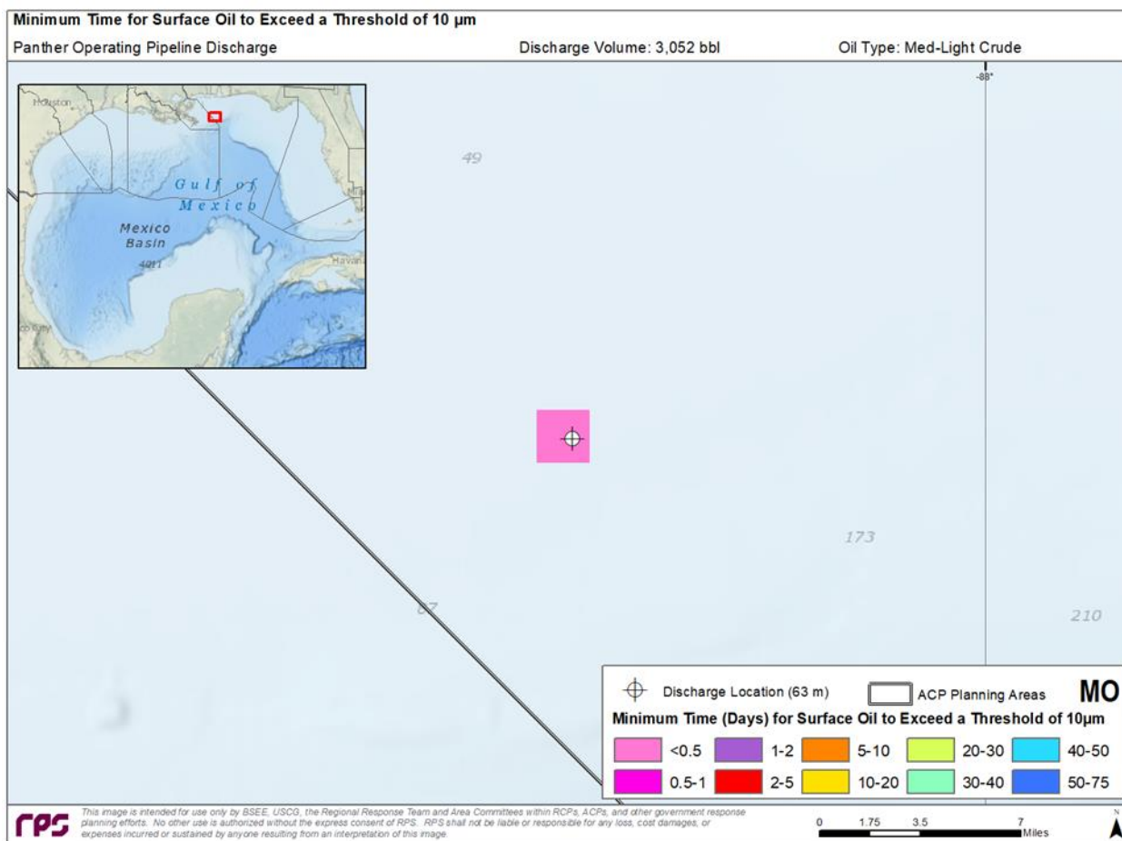
Figure 2. Minimum Travel Time for Oil on the Water Surface with Average Thickness greater than the Ecological Threshold of 10 \mu\text{m} .
