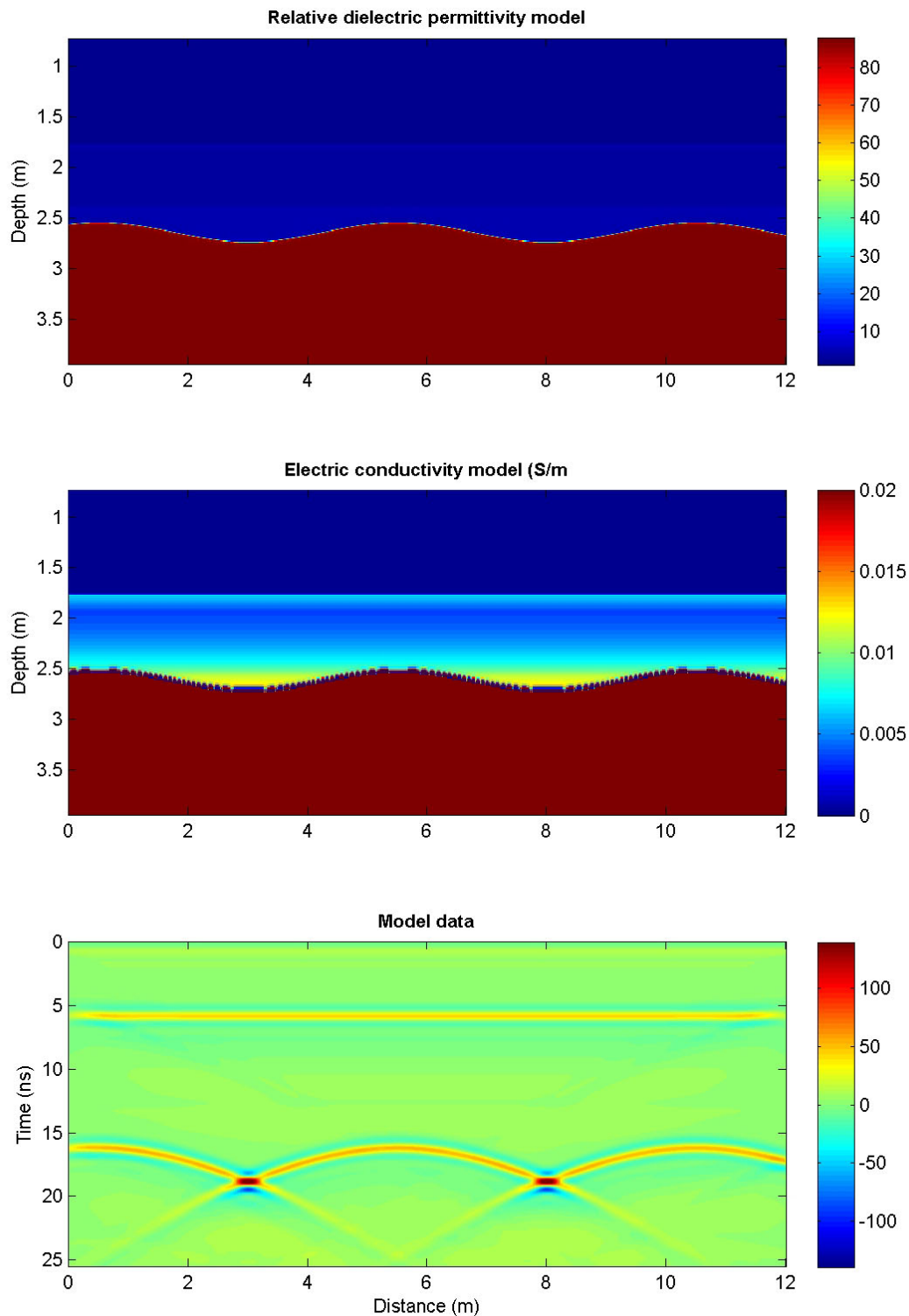
Figure 6-18 Electric property models and simulated GPR data for a laterally variable ice/water interface. The properties are based on our February test case used for Scenario 2
