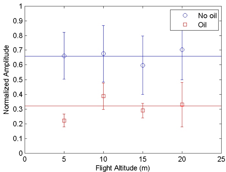
Figure 6-5 Summary of airborne radar results at speeds of 5N. The solid lines show the amplitudes predicted by numerical modeling. In all cases the mean amplitude of the oiled cell is significantly lower than that in the control cell.
