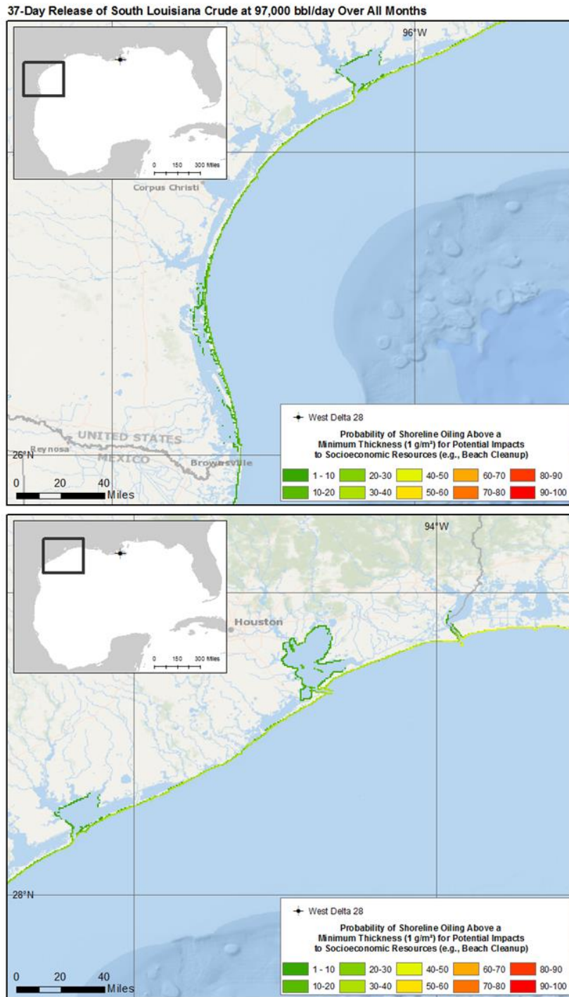
Figure 32: Scenario 2, GOM-WD28 – Shoreline Oiling Probabilities for Shoreline Oil (Including Weathered Tarballs) \geq 1 \text{ g/m}^2 ( 3.94 \times 10^{-5} \text{ in} , the Minimum Thickness for Potential Impacts to Socioeconomic Resources) along Texas and Louisiana Coasts
