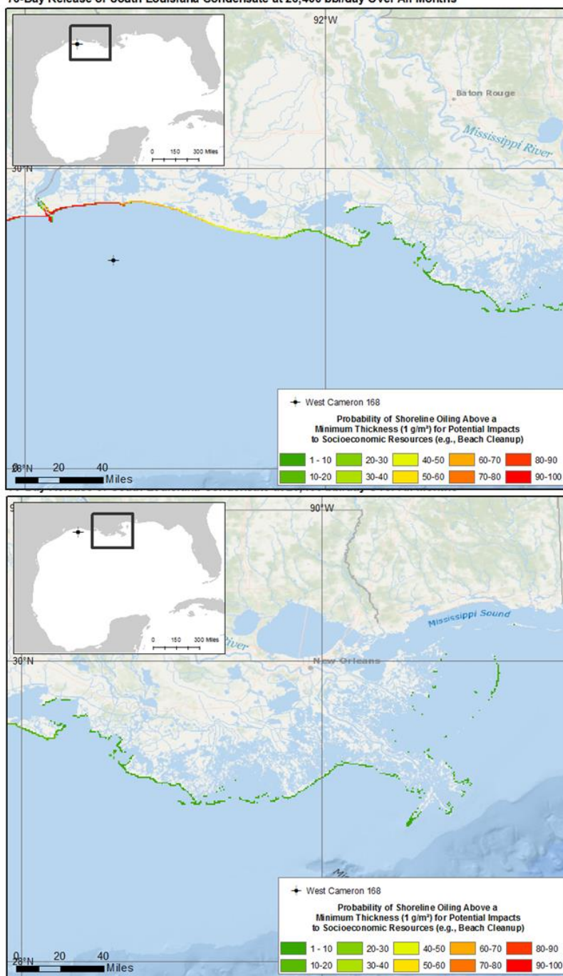
Figure 40: Scenario 3, GOM-WC168 – Shoreline Oiling Probabilities for Shoreline Oil (Including Weathered Tarballs) \geq 1 \text{ g/m}^2 ( 3.94 \times 10^{-5} in, the Minimum Thickness for Potential Impacts to Socioeconomic Resources) along Louisiana and Mississippi Coasts
