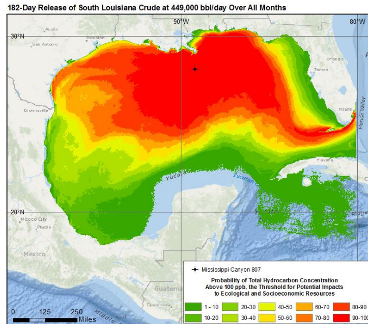
Figure 24: Scenario 1, GOM-MC807 – Probability of Total Hydrocarbon Concentration \geq 100 ppb (the Threshold above which Potential Impacts to Ecological and Socioeconomic Resources Could Occur)
