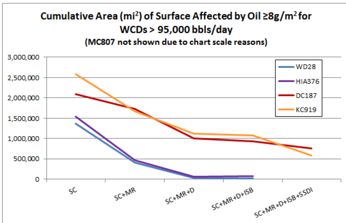
Figure ES 4: Effectiveness of Multiple Response Options for Cumulative Surface Area Oiled, WD28, HIA376, DC187, and KC919
