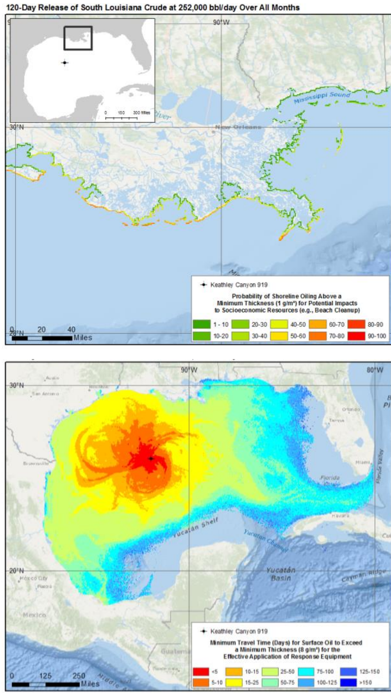
Figure 55: Scenario 5, GOM-KC919 Relief Well Only Scenario, 120-Day Discharge – Probability of Shoreline Oiling and Minimum Travel Times for Surface Oiling
