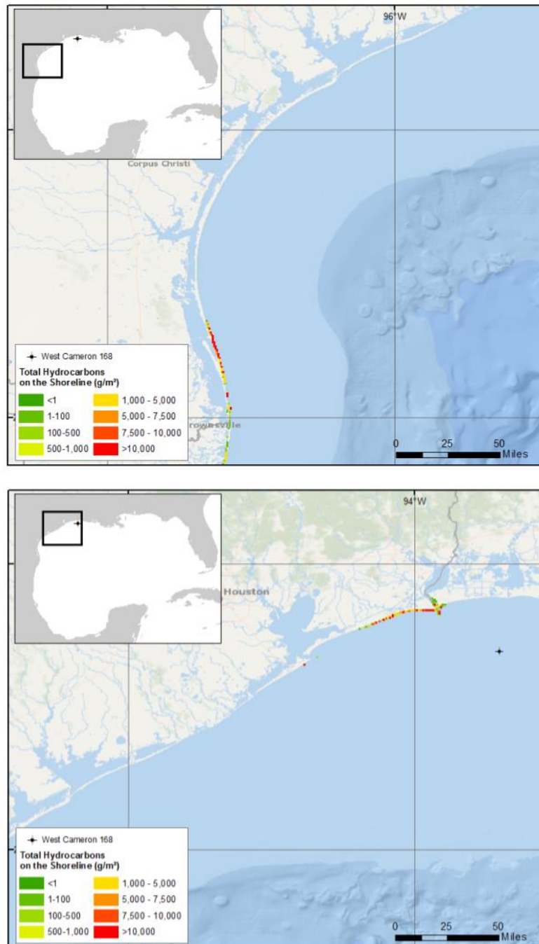
Figure 35: Scenario 3, GOM-WC168 Source Control, 21-Day Discharge – Shoreline Oil \geq 1 g/m 2 , including Weathered Tarballs
