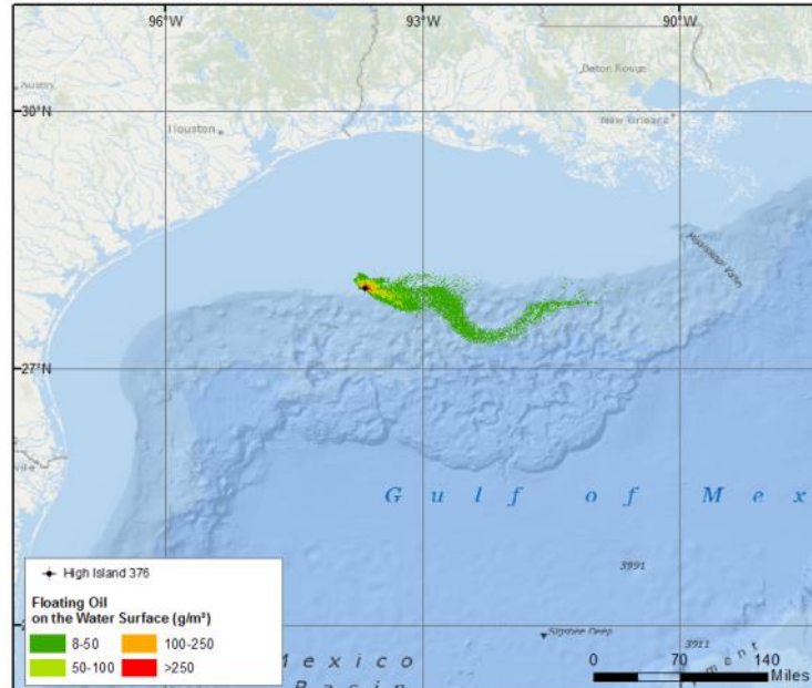
Figure 54: Scenario 4, GOM-HIA376 – Comparison Floating Oil Concentration ( \geq 8.0 g/m 2 ) over 66-Day SIMAP Model Simulation, Top Panel: Source Control (SC), Bottom Panel: Source Control, Mechanical Recovery, Surface Dispersants, and In Situ Burning (SC+MR+D+ISB)
