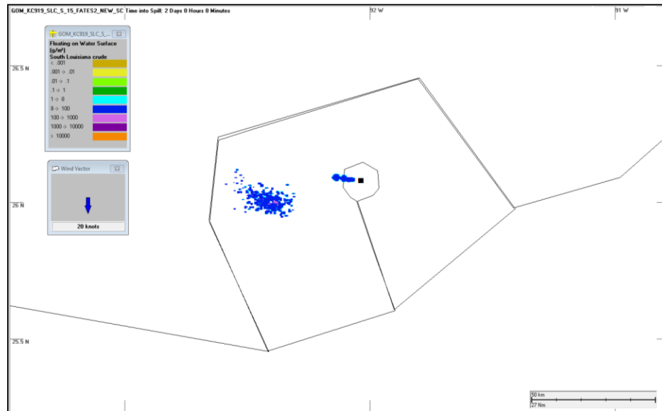
Figure 59: Scenario 5, GOM-KC919 Source Control – Floating Oil on Water Surface (g/m 2 ) at Day 2
