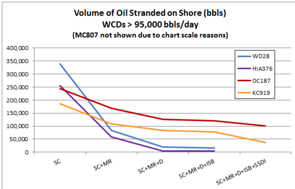
Figure ES 5: Effectiveness of Multiple Response Options for Oil Stranded on Shore, WD28, HIA376, DC187, and KC919
