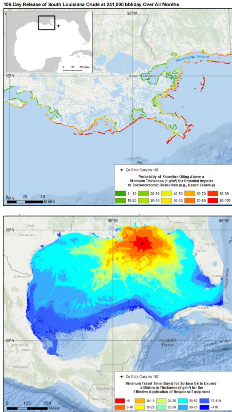
Figure 67: Scenario 6, GOM-DC187 Relief Well Only Scenario, 106-Day Discharge – Probability of Shoreline Oiling and Minimum Travel Times for Surface Oiling
