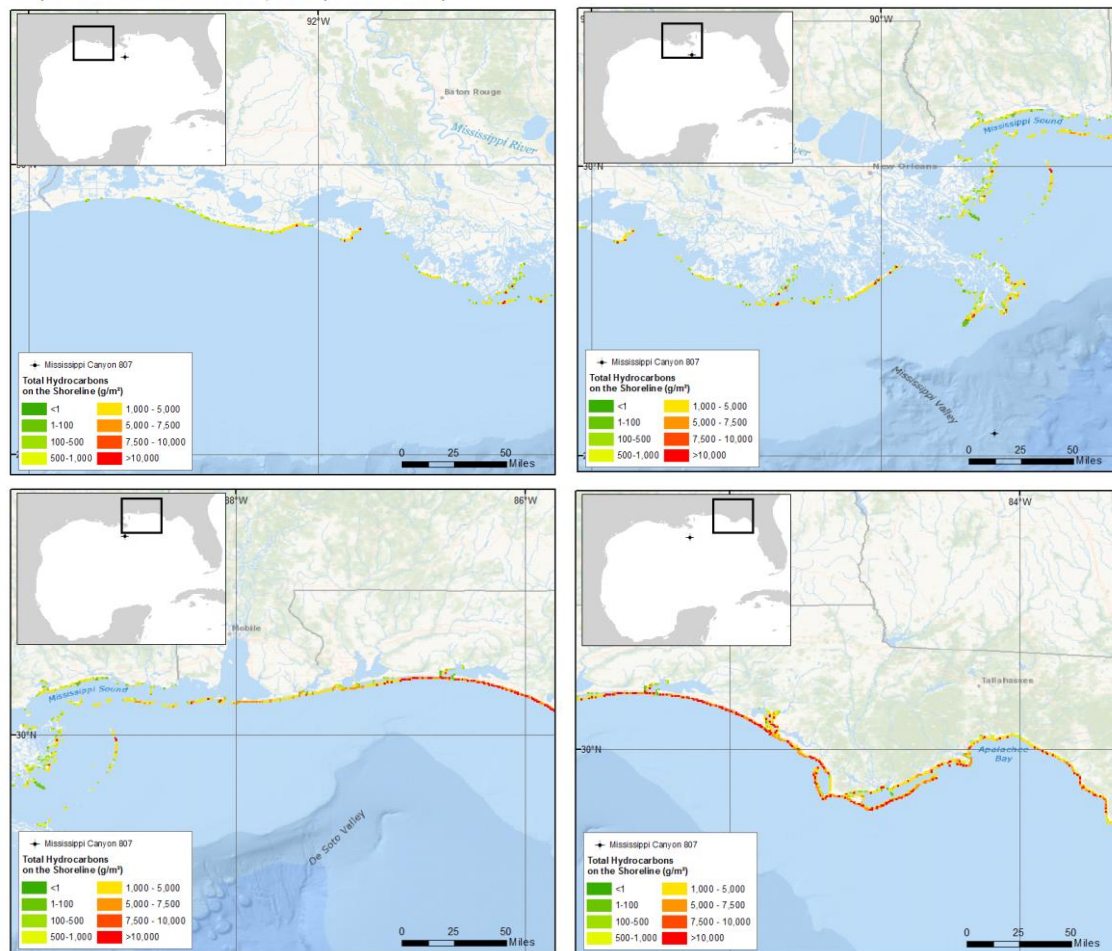
45-Day Release of South Louisiana Crude at 449,000 bbl/day - Source Control Only
