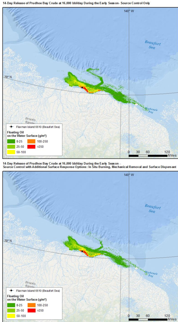
Figure 128: Scenario 10, Arctic-FI6610 Early Season – Comparison Floating Oil Concentration ( \geq 8.0 g/m 2 ) over 59-Day SIMAP Model Simulation, Top Panel: Source Control (SC), Bottom Panel: Source Control, Mechanical Recovery, Surface Dispersants, and In Situ Burning (SC+MR+D+ISB)
