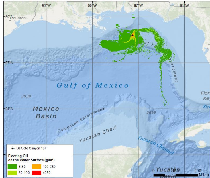
Figure 78: Scenario 6, GOM-DC187 – Comparison Floating Oil Concentration ( \geq 8.0 \text{ g/m}^2 ) over 90-Day SIMAP Model Simulation, Top Panel: Source Control (SC), Bottom Panel: Source Control, Mechanical Recovery, Surface Dispersants, and In Situ Burning (SC+MR+D+ISB+SubD)
