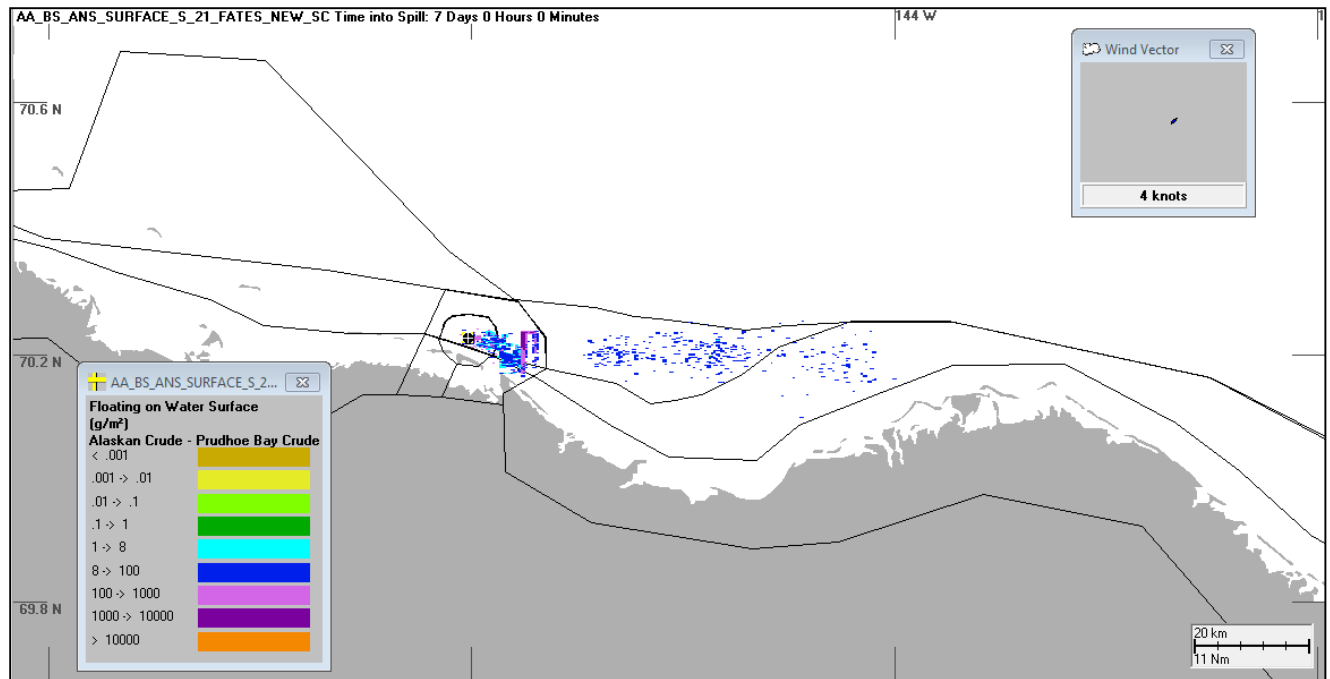
Figure 121: Scenario 10, Arctic-FI6610 Early Season Source Control – Floating Oil on Water Surface (g/m²) at Day 7
