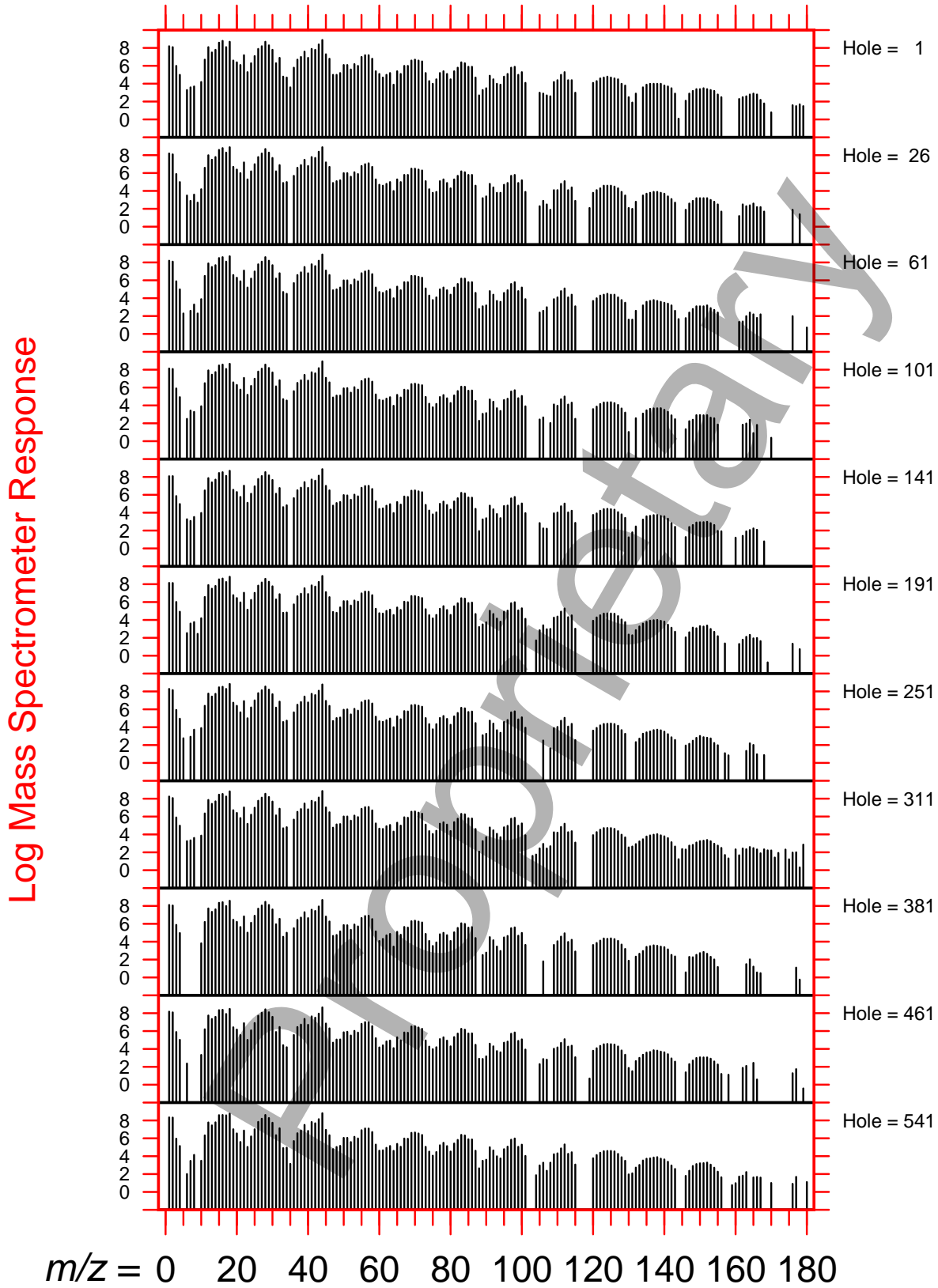
Figure 26: Oil Spectra
