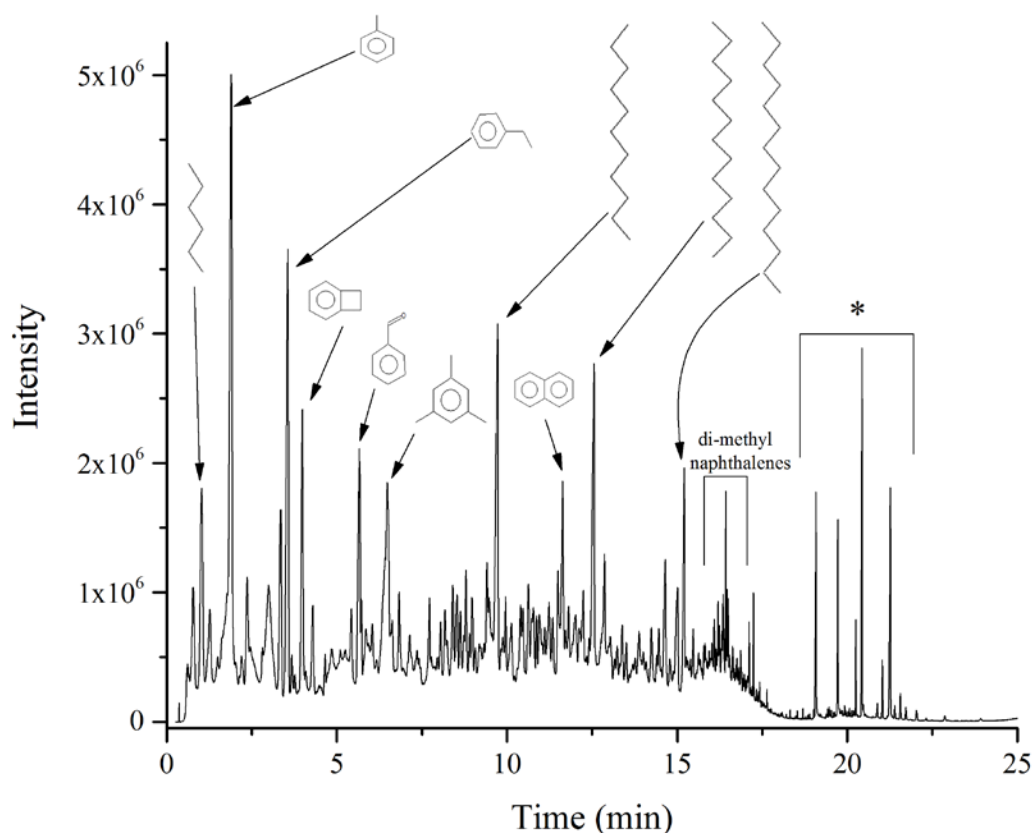
Fig. 79- Spectra from exhaust samples gathered in a sorbent tube for 25% emulsified ANS burned in a laboratory spray plume with \dot{m}_{\text{Air}} = 2.9 \times 10^{-4} \text{ kg/s} , \dot{V}_{\text{Oil}} = 23.2 \text{ mL/min} (see Table 3). * denotes major peaks identified in Fig. 78 from the baseline neat ANS crude
