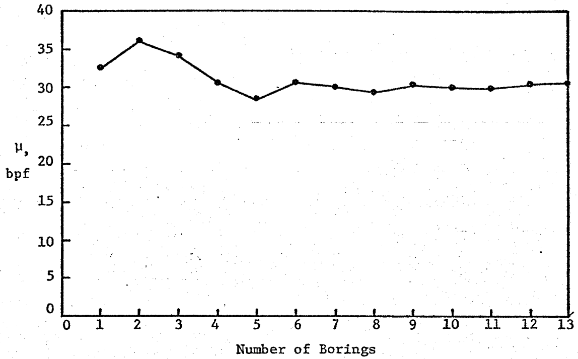
FIG. 3. - Mean of SPT Values vs. Number of Borings (1ft. = 0.3048 m)
