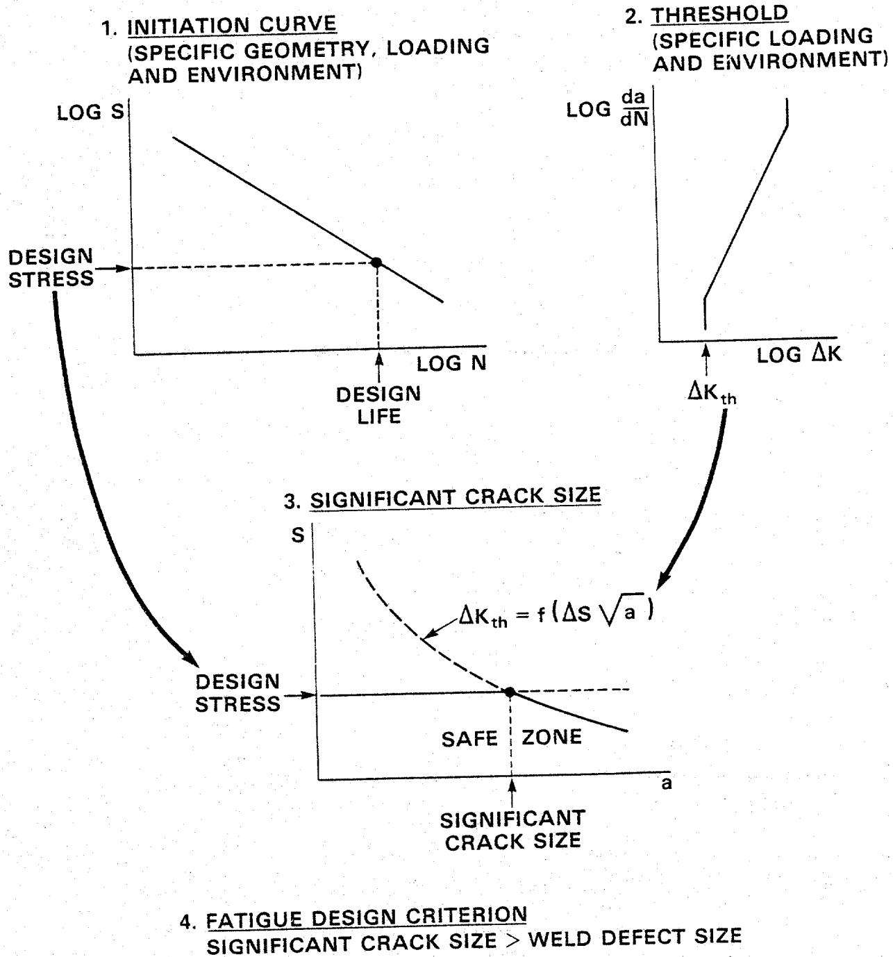
Fig. 3 — Scheme for integrating the \Delta K_{th} concept into traditional fatigue design procedures for offshore structures [11].
