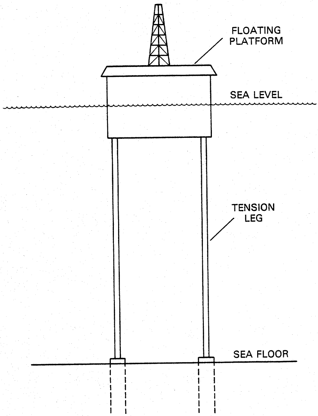
Fig. 1 — Schematic view of a tension leg platform (TLP).
