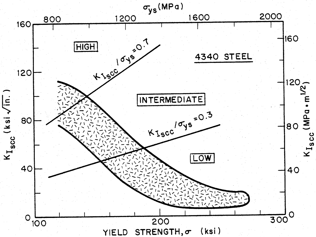
Fig. 5 — Influence of yield strength ( \sigma_{ys} ) on K_{I_{SCC}} for a high-strength steel [25]. SCC sensitivity is categorized on the basis of K_{I_{SCC}}/\sigma_{ys} ratios.
