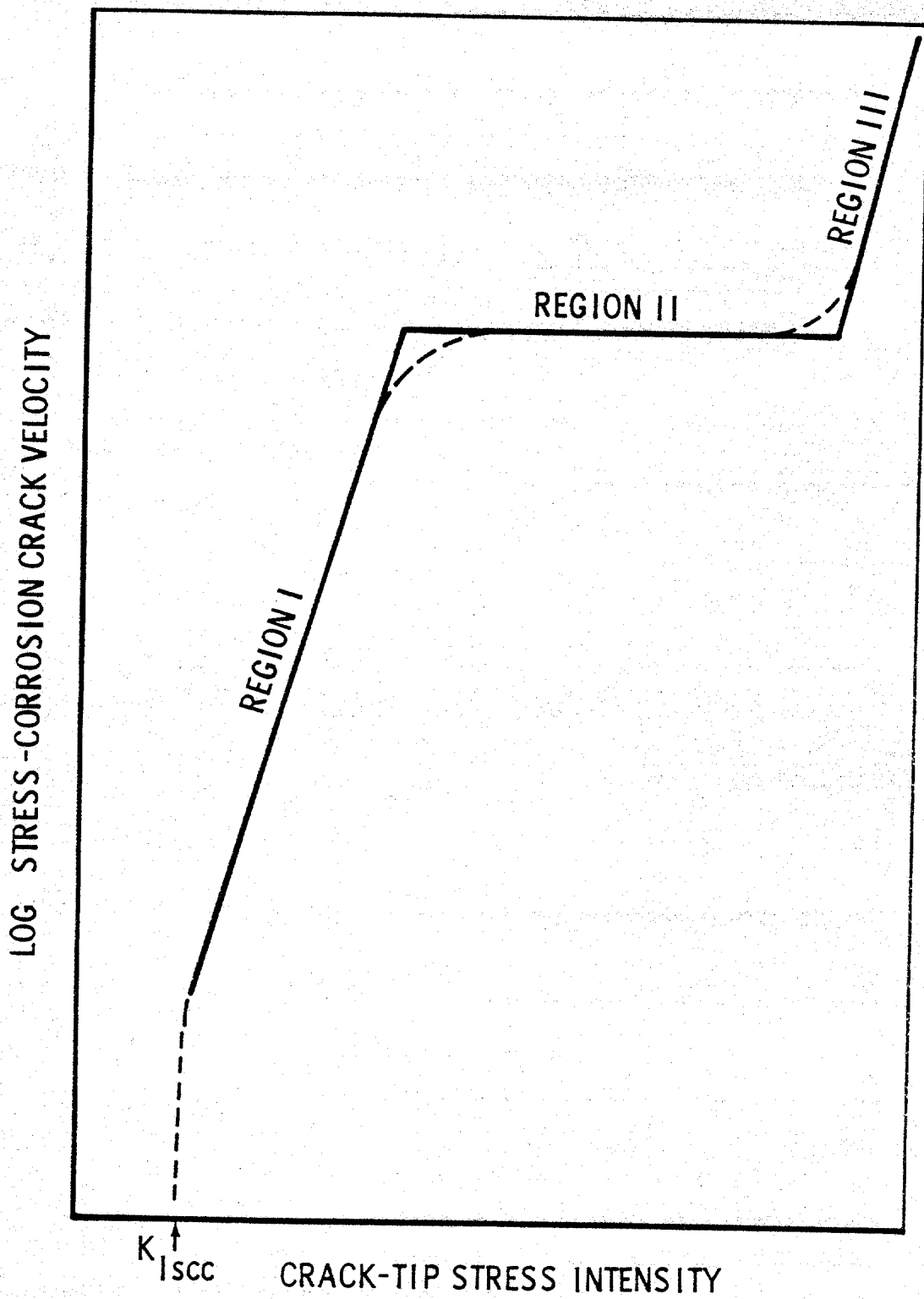
Fig. 4 — Typical relationship between stress-corrosion crack growth rate ( da/dt ) and stress-intensity-factor K_I . The Region I threshold defines K_{Isc} .
