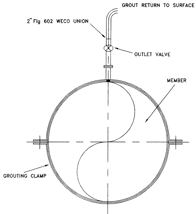
VIEW B-B
