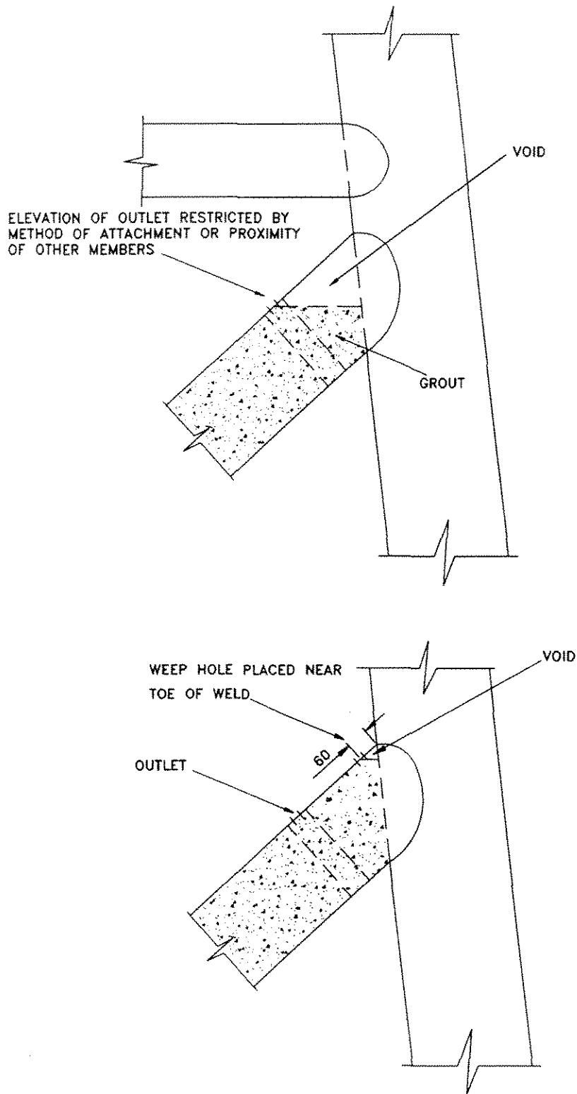
Figure 4.4 – OUTLET DETAILS
