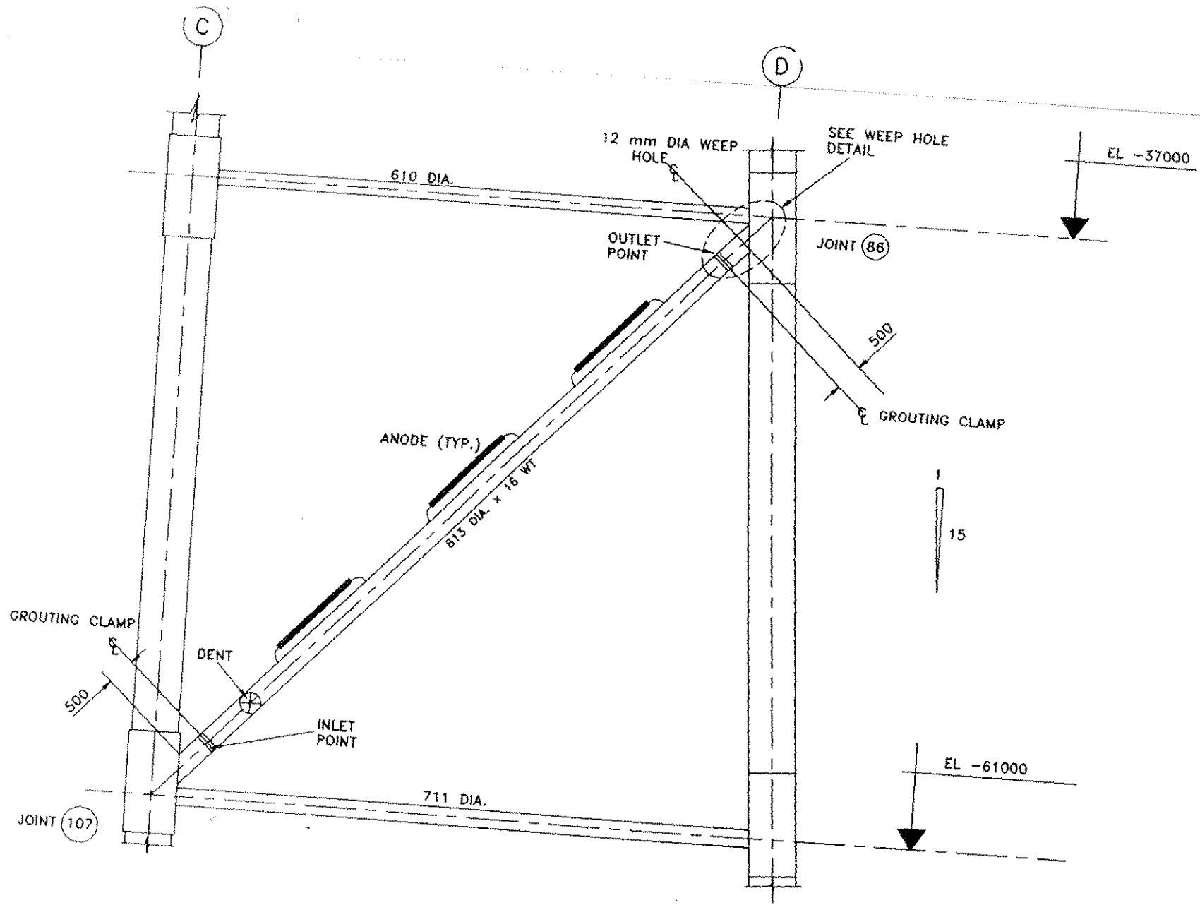
Figure 4.7 ELEVATION ON MEMBER 1
