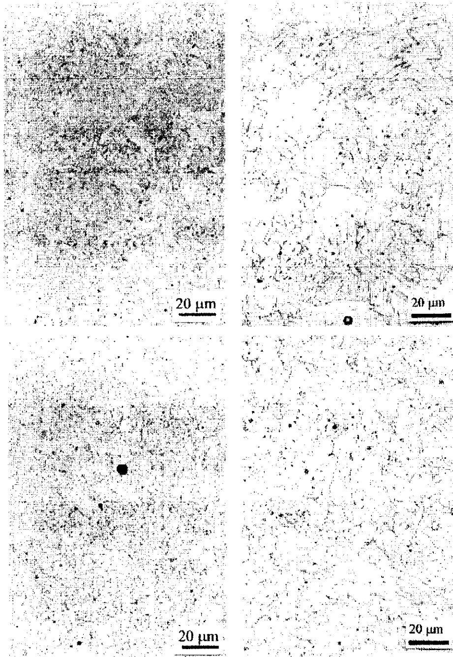
Figure 51: Reheated steel weld metal microstructures from 1T2B2 (left) and 1F3 (right) V-groove welds. The coarse-grained reheated zone appears at top, the fine-grained reheated zone appears in the bottom two photomicrographs.
