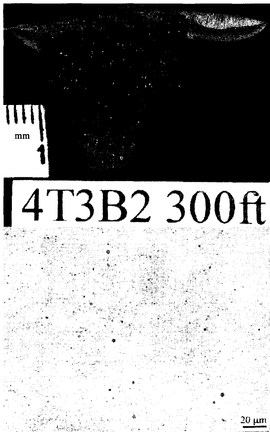
Figure 45: Macro-section and top bead microstructure from 4T3B2 V-groove weld.
