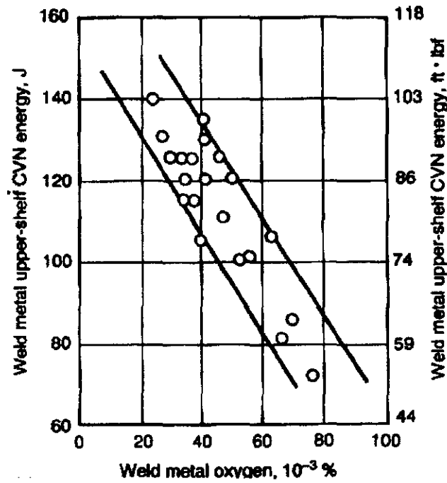
Figure 13: Weld metal upper shelf toughness as a function of weld metal oxygen content. (Ahblom 1984).
