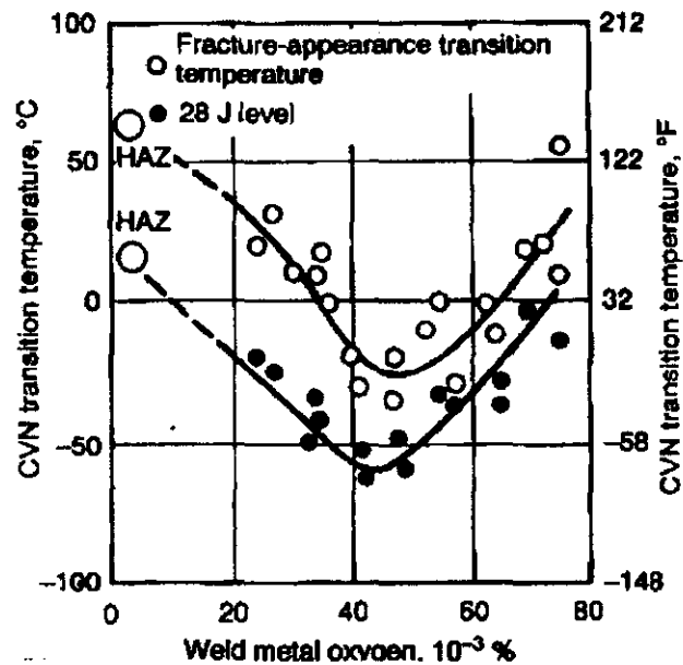
Figure 14: Charpy transition temperature as a function of weld metal oxygen content. (Ahblom 1984).
