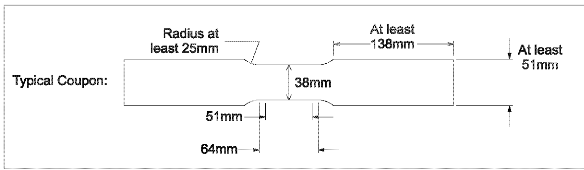
Figure 4.14 Typical Coupon Location and Dimensions
