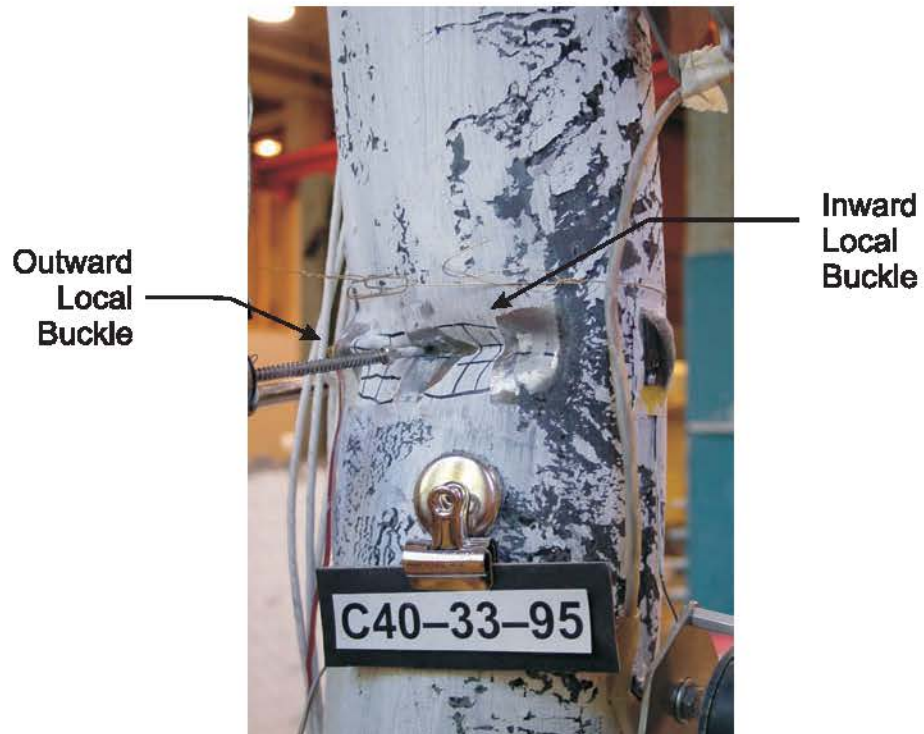
Figure 5.51 Side View of Local Buckle at Mid-height (Load Step -2), Specimen C40-33-95
