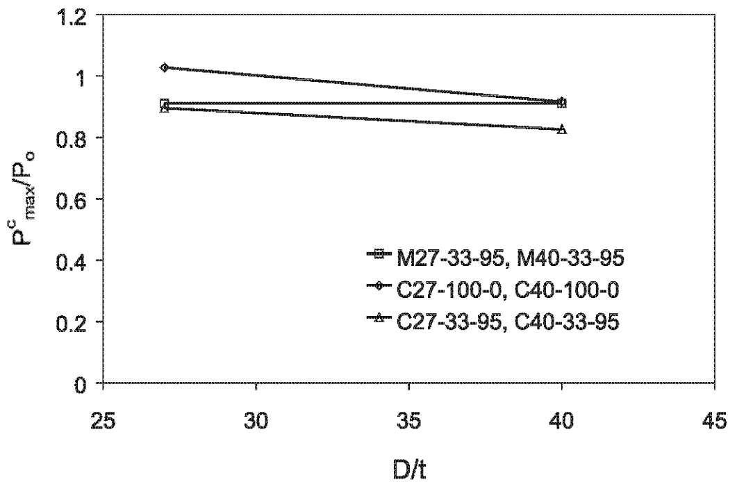
Figure 6.7 Effect of D/t on Peak Compression Axial Load
