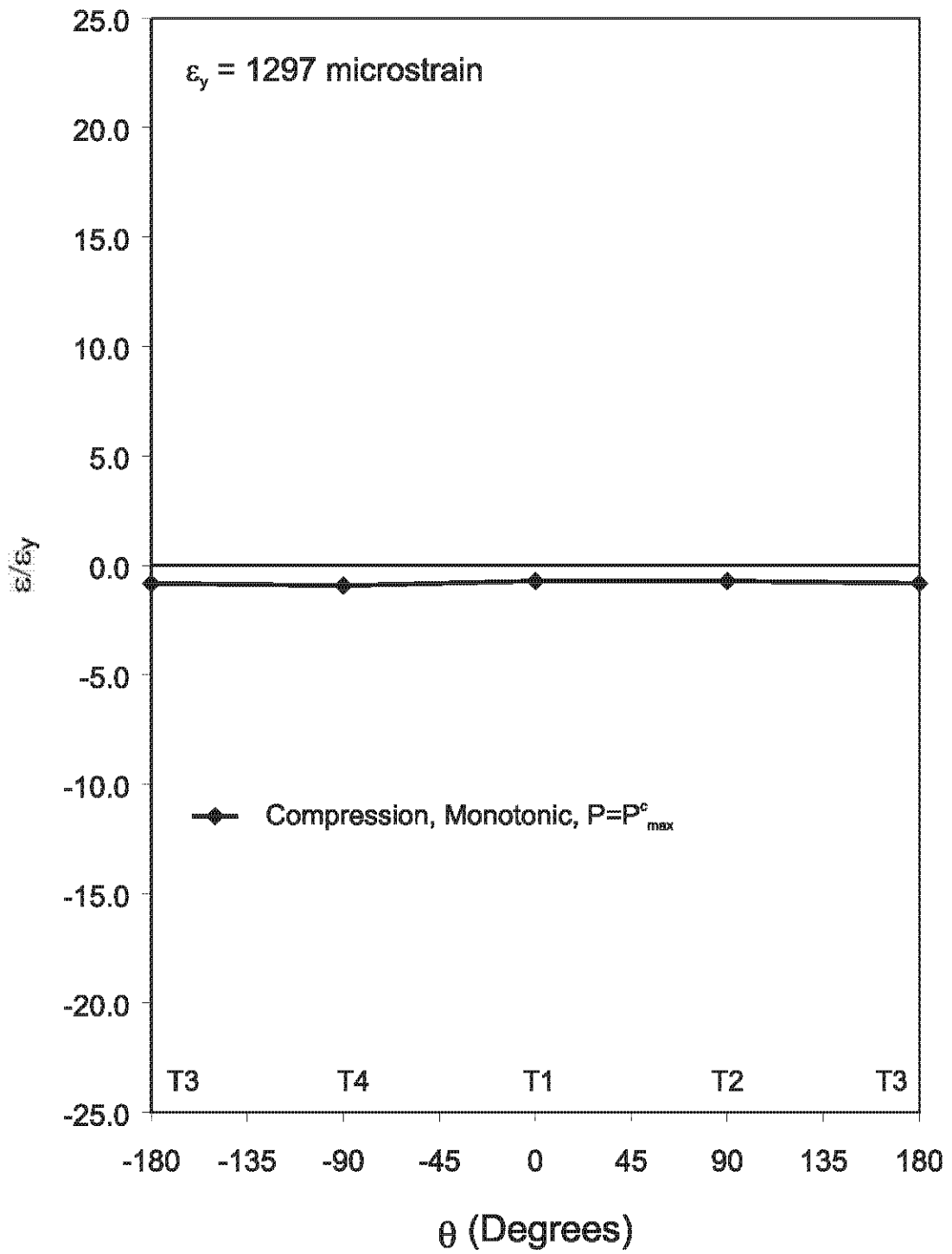
Figure 5.36 Strain Distribution of Cross Section at Upper Quarter-point, Specimen M27-33-95
