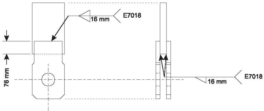
(b) Assembled Female Clevis
