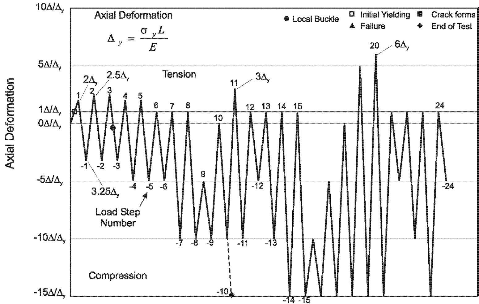
Figure 5.14 Displacement History with Events of Interest Noted, Specimen C27-100-0
