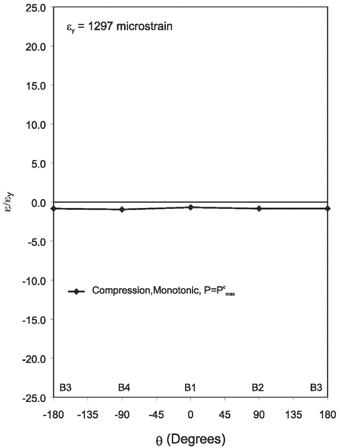
Figure 5.35 Strain Distribution of Cross Section at Lower Quarter-point, Specimen M27-33-95
