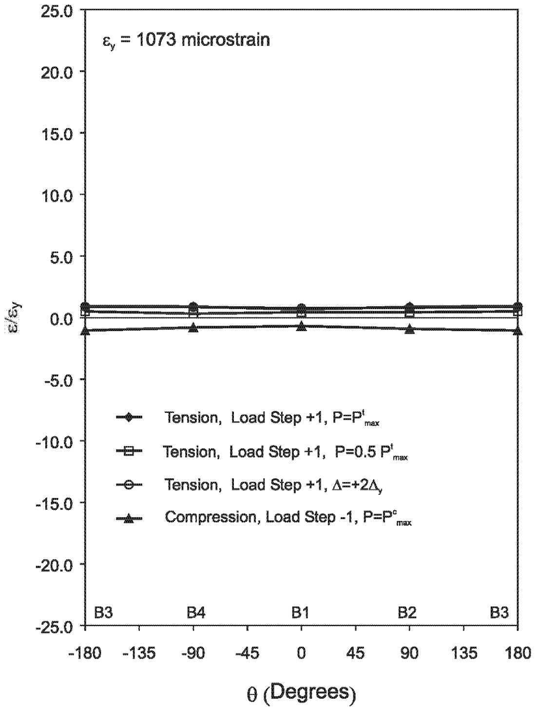
Figure 5.67 Strain Distribution of Cross Section at Lower Quarter-point, Specimen C40-00-95
