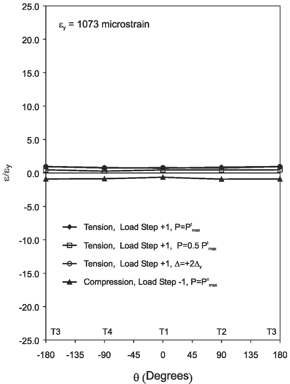
Figure 5.68 Strain Distribution of Cross Section at Upper Quarter-point, Specimen C40-00-95
