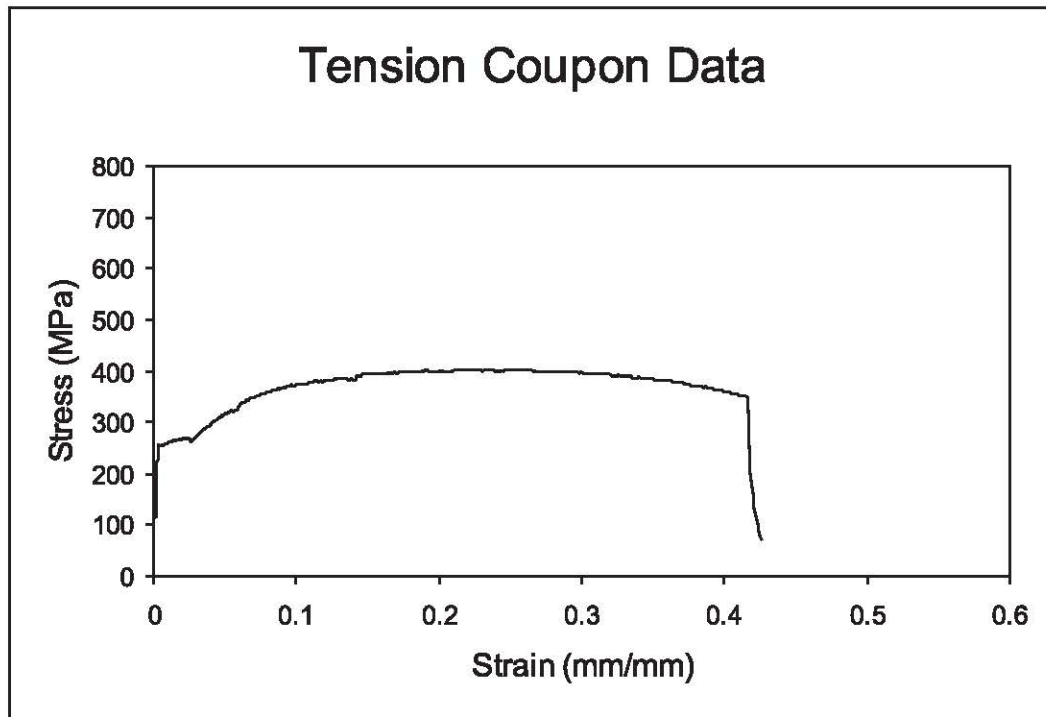
Figure 4.18 Stress-Strain Plot for D/t = 27 , Annealed
