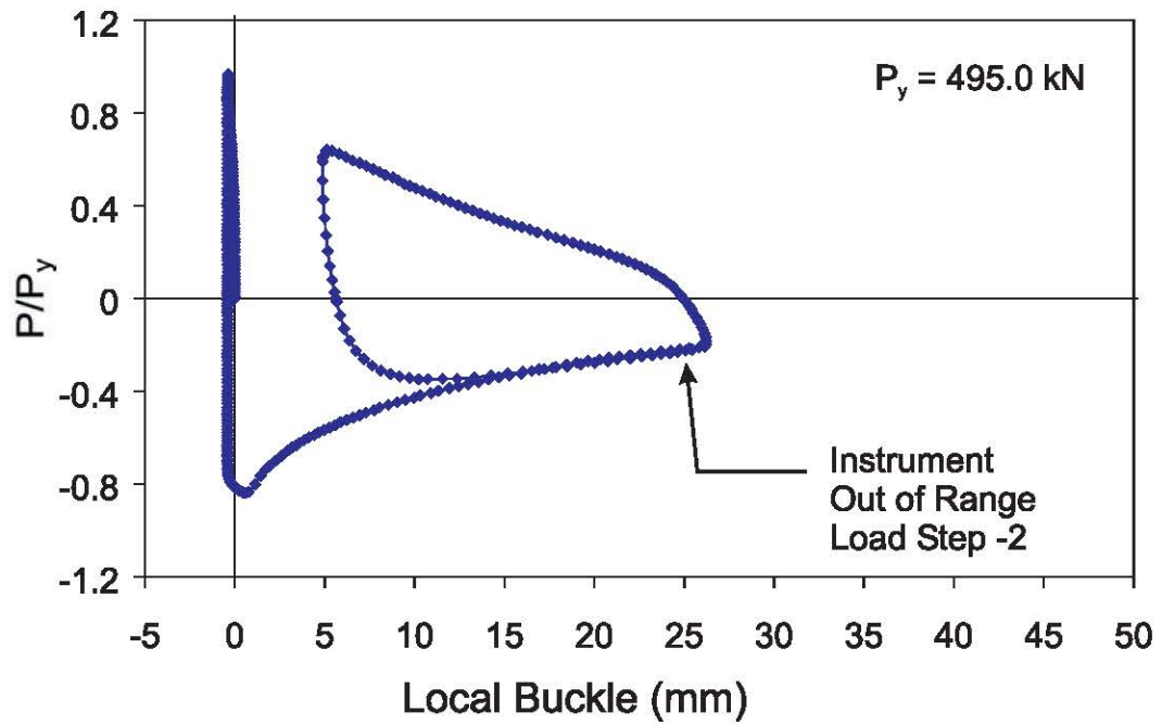
Figure 5.84 Measured Local Displacement of Buckle in Corrosion Patch, Specimen C27-33-95
