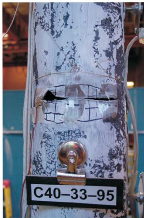
Figure 5.55 Through Thickness Cracking Across Local Buckle (Load Step +4), Specimen C40-33-95
