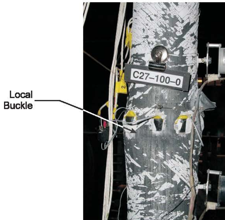
Figure 5.18 Front View of Local Buckle at Mid-height on Southern Face (Load Step -3), Specimen C27-100-0
