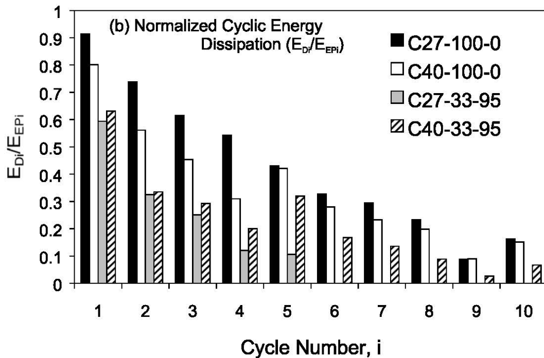
Figure 6.13 Effect of Diameter to Thickness Ratio ( D/t ) on Deterioration of Energy Dissipation per Cycle
