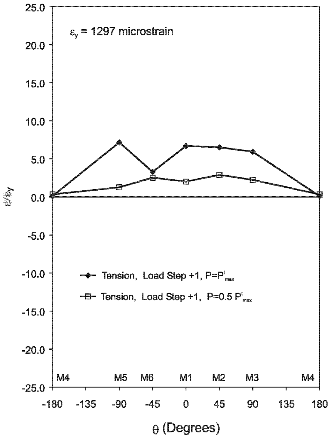
Figure 5.96 Strain Distribution of Cross Section at Mid-height, Specimen C27-33-311
