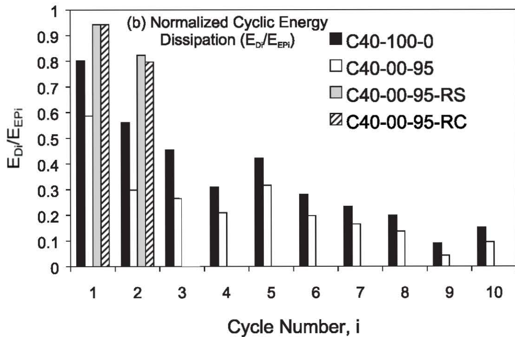
Figure 6.43 Effect of Repair on Energy Dissipation
