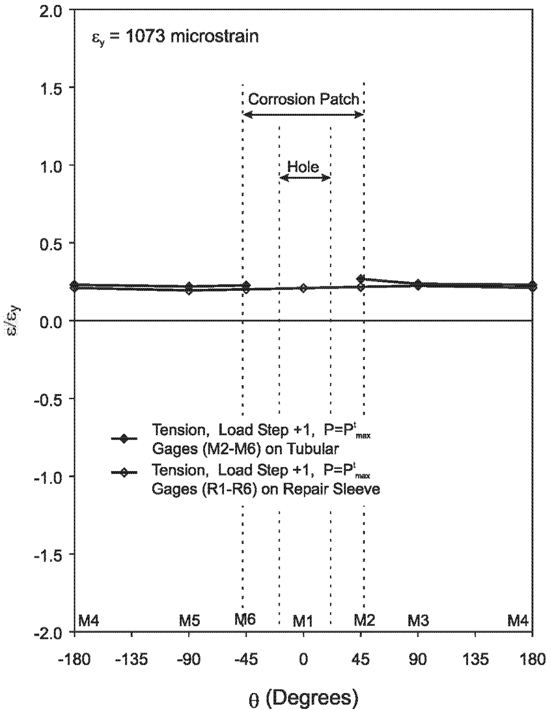
Figure 5.105 Strain Distribution of Cross Section at Mid-height on Tubular and Repair Sleeve at Peak Tension Load ( P_{max}^i ), Specimen C40-00-95-RS
