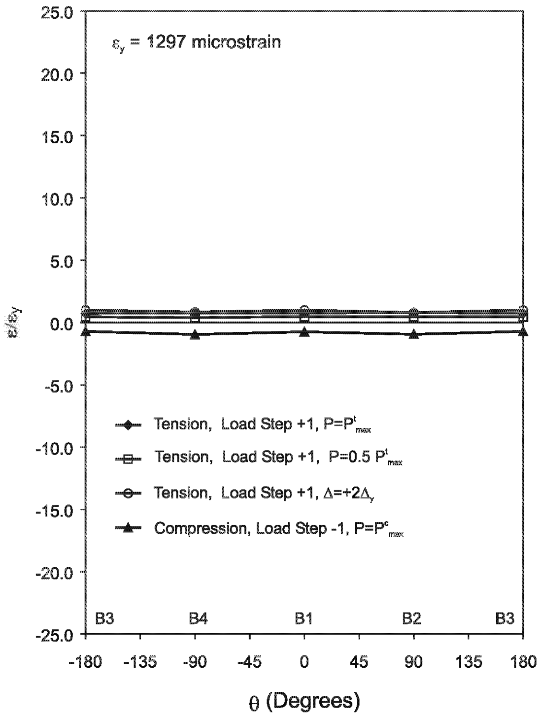
Figure 5.79 Strain Distribution of Cross Section at Lower Quarter-point, Specimen C27-33-58
