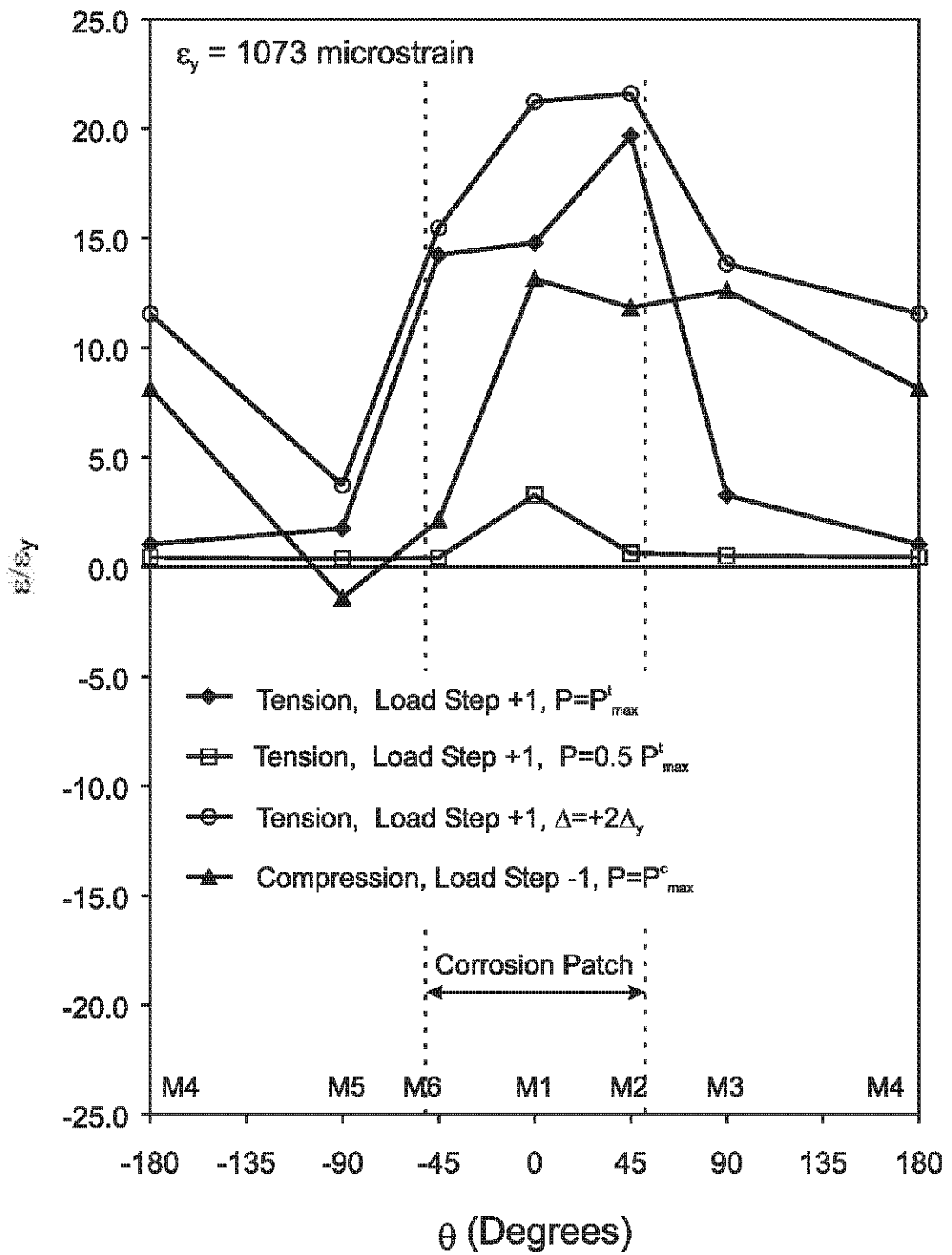
Figure 5.57 Strain Distribution of Cross Section at Mid-height, Specimen C40-33-95
