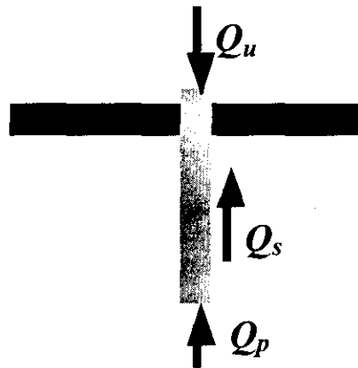
Figure 2.7 The ultimate axial pile response
