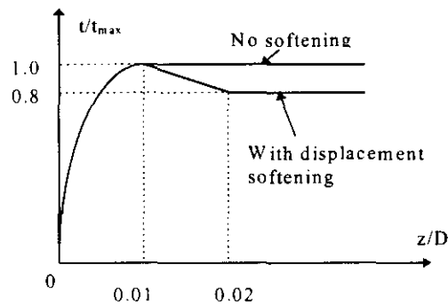
Fig. 4.1 t-z curves
