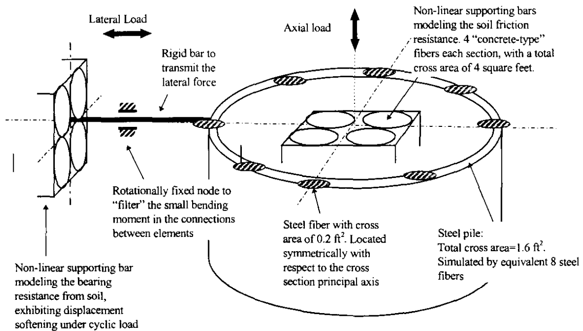
Figure 3.2 Details of the configuration of elements and sub-elements at pile node
