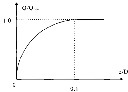
Fig 4.2 q-z curve
