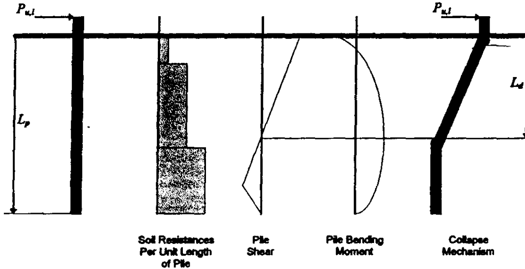
Figure 2.6 Illustration of collapse mechanism for laterally loaded pile
