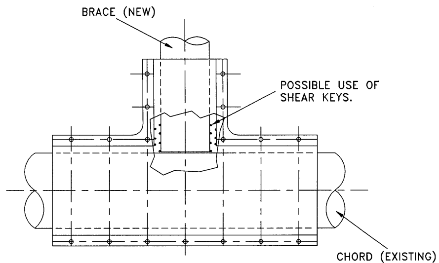
b) Attachment of a new member.
