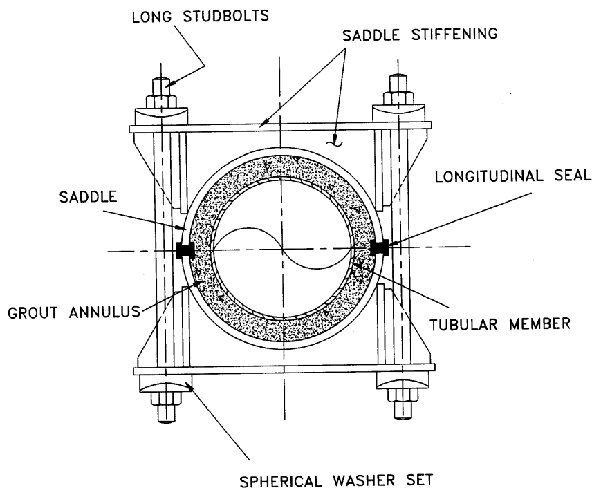
Figure 9.8: Typical stressed grouted clamp
