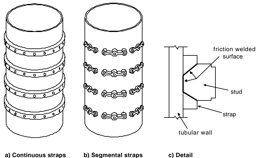
Figure 9.10: Stud/strap connection
