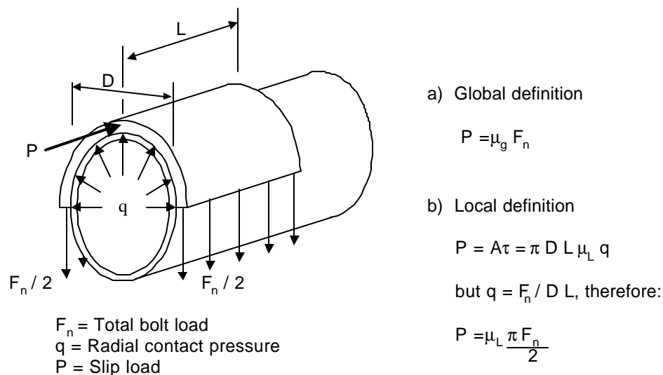
Figure 9.14: Definitions of coefficients of friction
