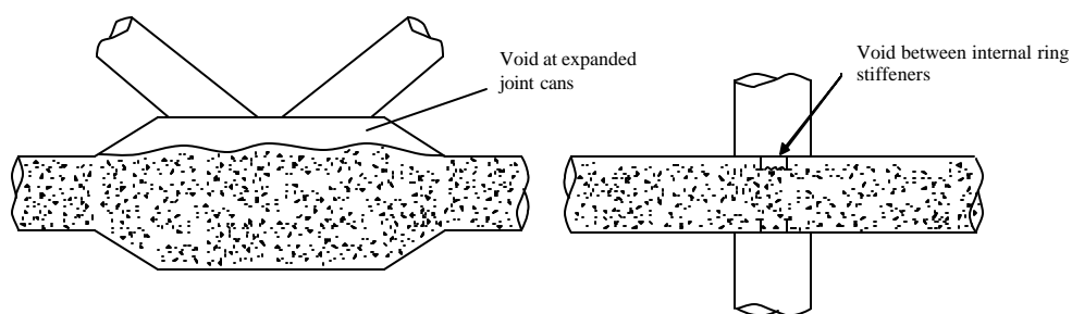
Figure 11.2: Void formation at joints
