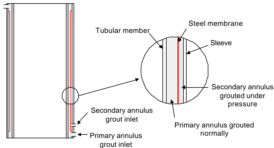
Figure 9.11: Pressurized grouted connection
