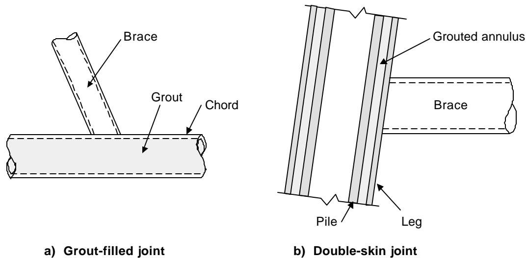
Figure 11.1: Grout-filled and double-skin joints
