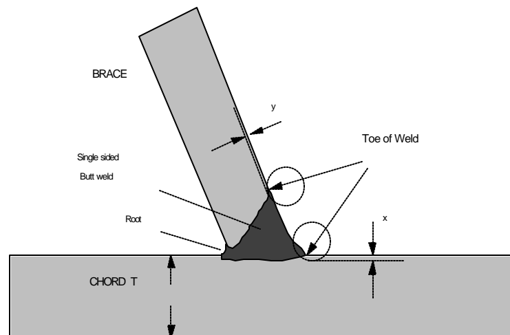
Figure 12.1: A typical application of toe grinding
