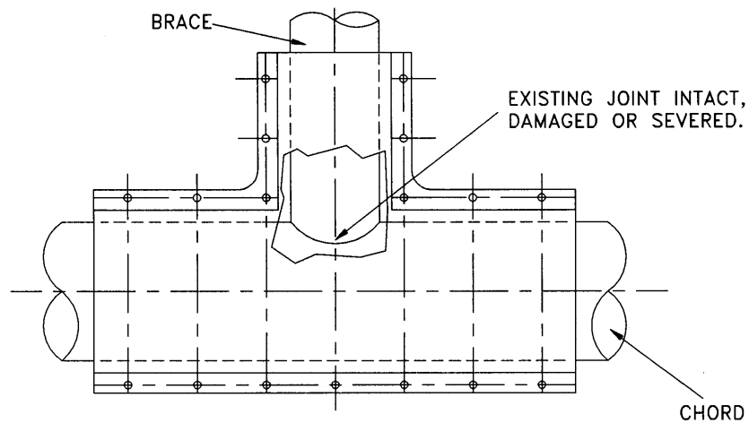
a) Repair of an existing tubular joint.
