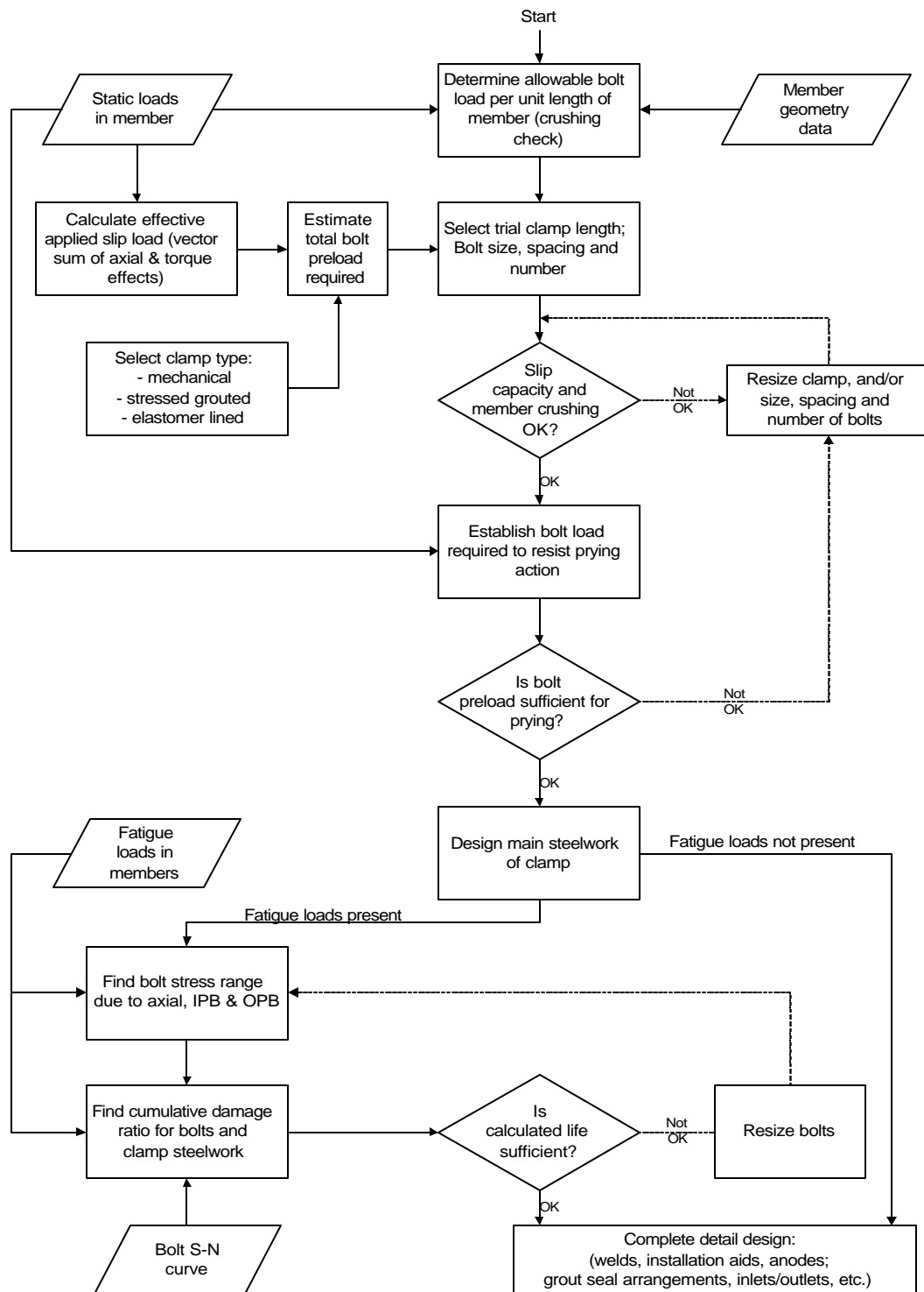
Figure 9.13: Design process for stressed clamps
