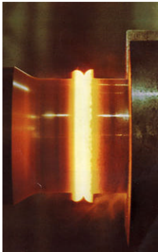
Figure 8.2: Friction stud welding
