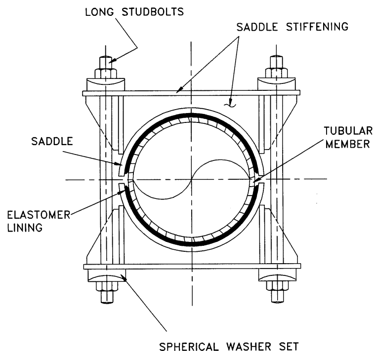
Figure 9.9: Typical stressed elastomer lined clamp
