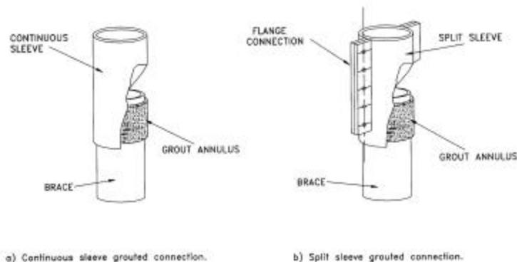
Figure 9.5: Examples of typical unstressed grouted sleeve connections
