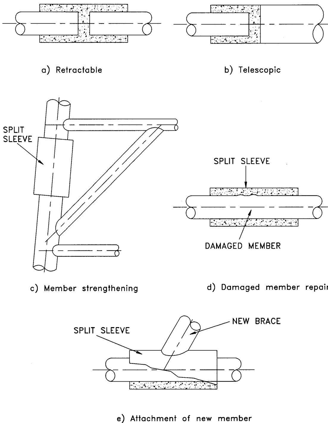
Figure 9.7: Some applications of unstressed grouted sleeve connections
