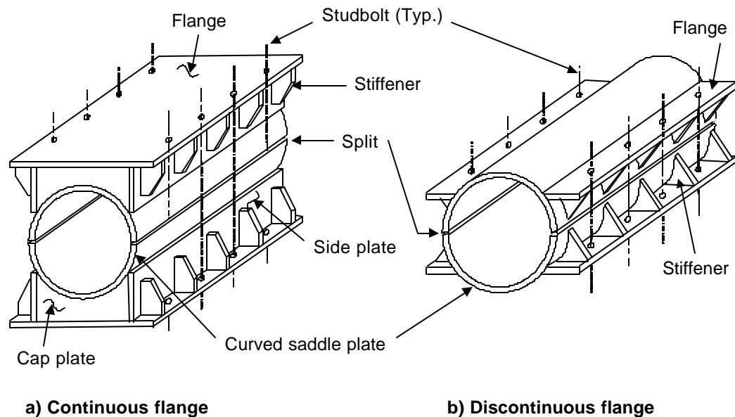
Figure 9.1: Clamp terminology
