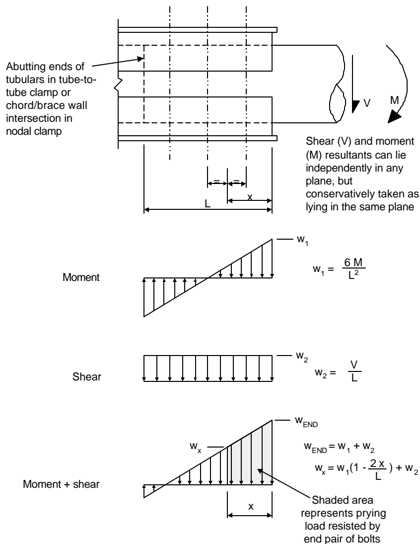
Figure 9.13: Traditional approach for estimating prying forces
