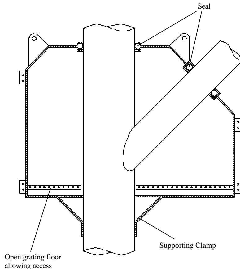
Figure 7.2: Hyperbaric welding habitat
