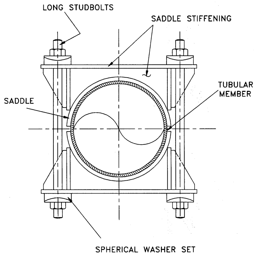
Figure 9.2: Typical stressed mechanical clamp
