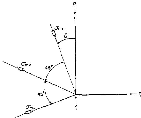
FIG. 8. Stress sensor rosette used to determine the magnitude and direction of the principal stresses.
