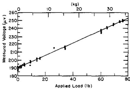
FIG. 3. Load sensitivity for the uniaxial brass ice stress sensor from direct loading tests.
