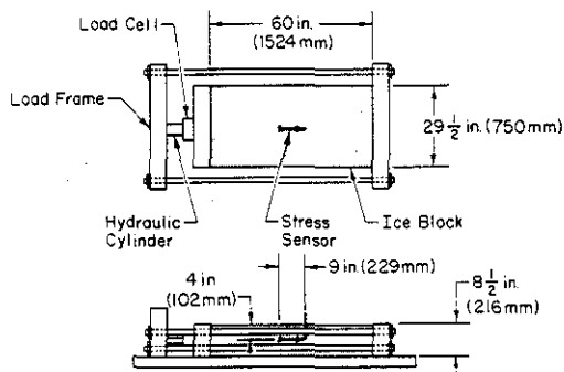
FIG. 2. Experimental test setup for the load frame, ice block, and stress sensor.
