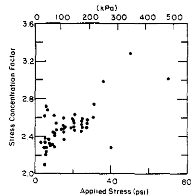
FIG. 7. Stress concentration factor as a function of the applied ice stress for \theta = 0^\circ configuration.
