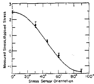
FIG. 5. Measured sensor stress to applied ice-stress ratio as a function of stress sensor orientation to the principal stress direction.
