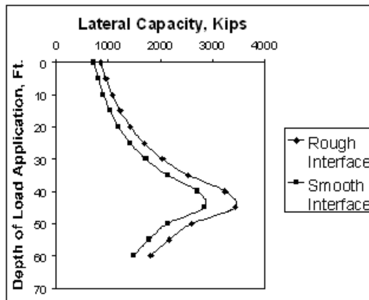
Lateral Capacity of a Suction Caisson vs. Depth of Load Application ( L=60 ft., D=15 ft., s_{uc}=50 psf, s_{ul}=10 psf/ft.)
