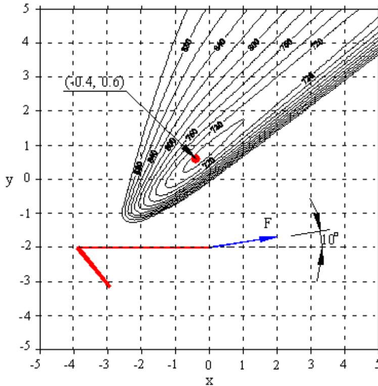
Figure 14. Contours of Anchor Resultant Force for 10° Force Inclination Angle
