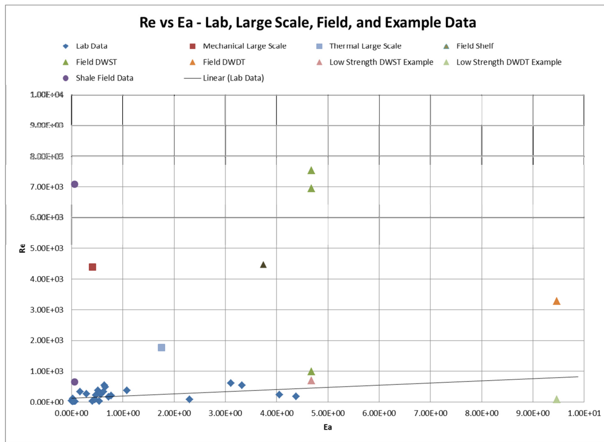
FIGURE 10: CORRELATION SENSITIVITY
