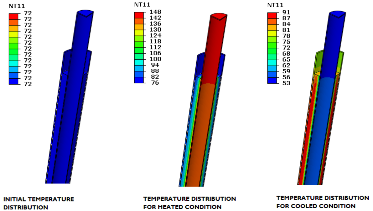
FIGURE 37: LARGE SCALE TEMPERATURE DISTRIBUTIONS
