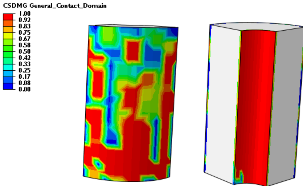
CONTACT DAMAGE AT ESTIMATED FAILURE
