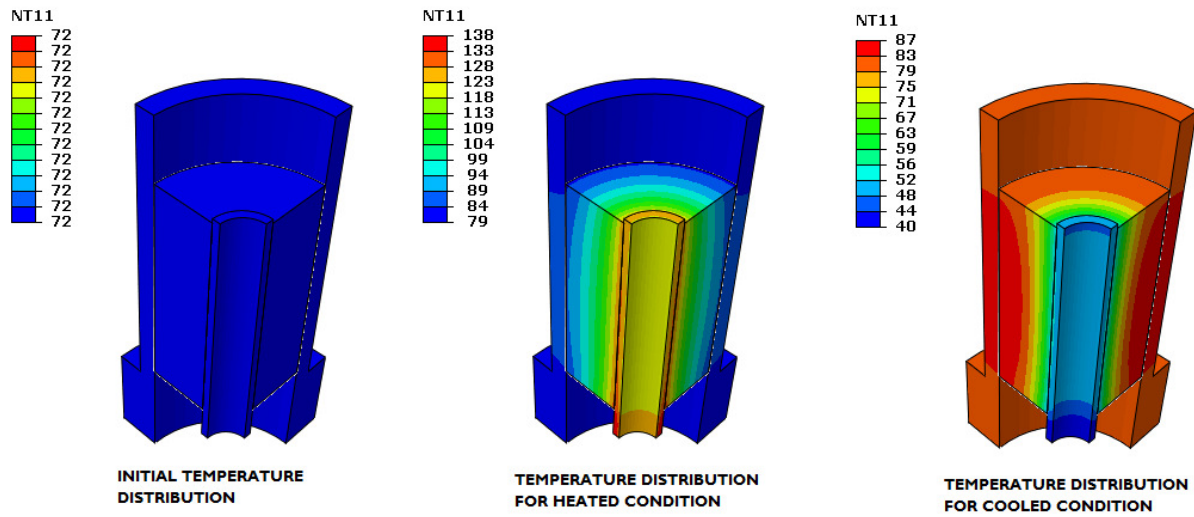
FIGURE 36: SMALL SCALE TEMPERATURE DISTRIBUTIONS (STEEL OUTER PIPE)
