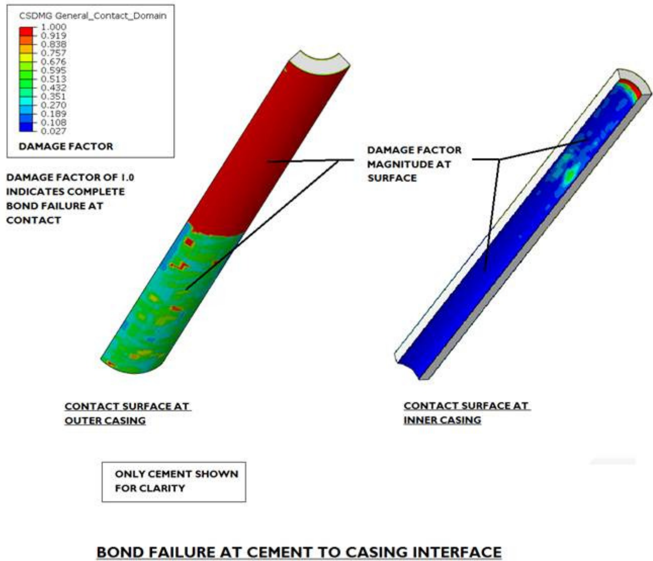
FIGURE 12: DEBONDING
