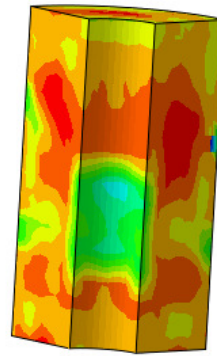
FIGURE 50: SMALL SCALE STRESS CONTOURS AT FAILURE FOR THERMAL TESTS (CPVC)
