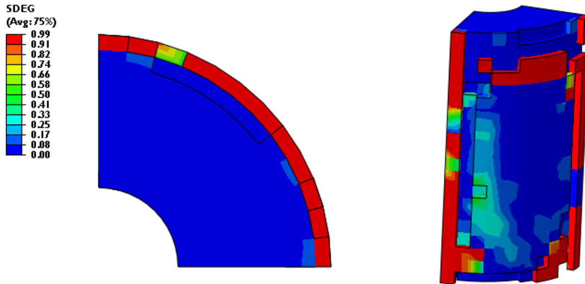
ELEMENT DAMAGE AT ESTIMATED FAILURE
