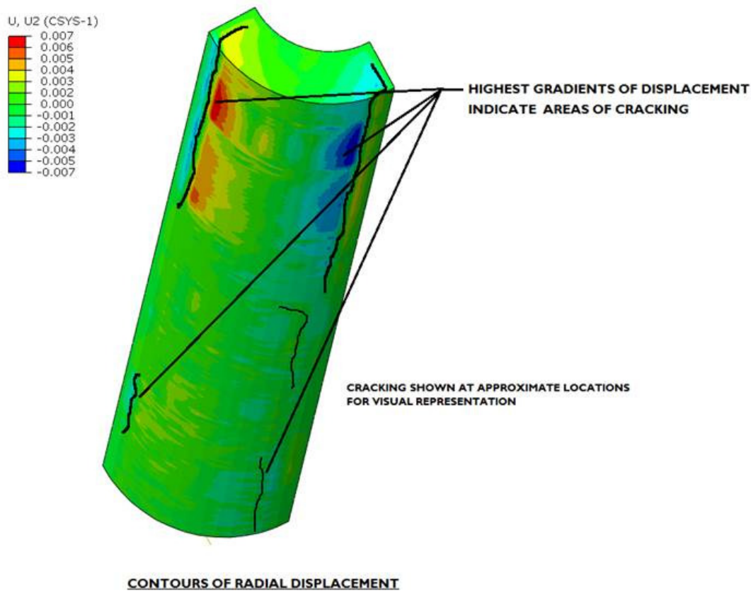
FIGURE 11: DISPLACEMENT GRADIENTS
