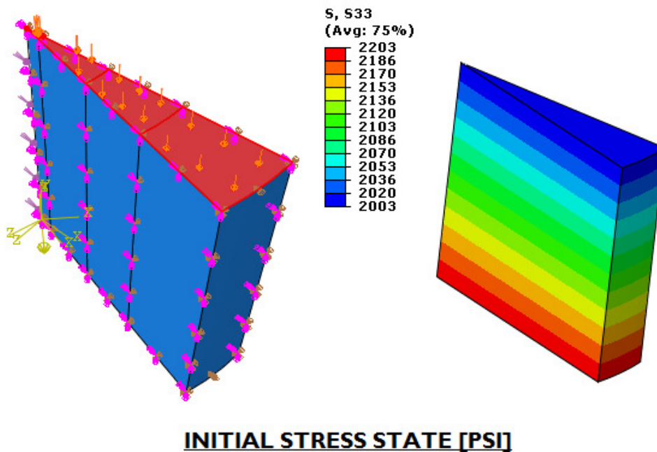
FIGURE 30: INITIAL VERTICAL STRESS STATE FOR DOWN-HOLE SYSTEM
