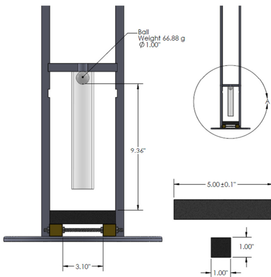
FIGURE 15: IMPACT SETUP
