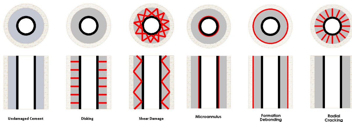
FIGURE 3: CEMENT SHEATH FAILURE MODES
