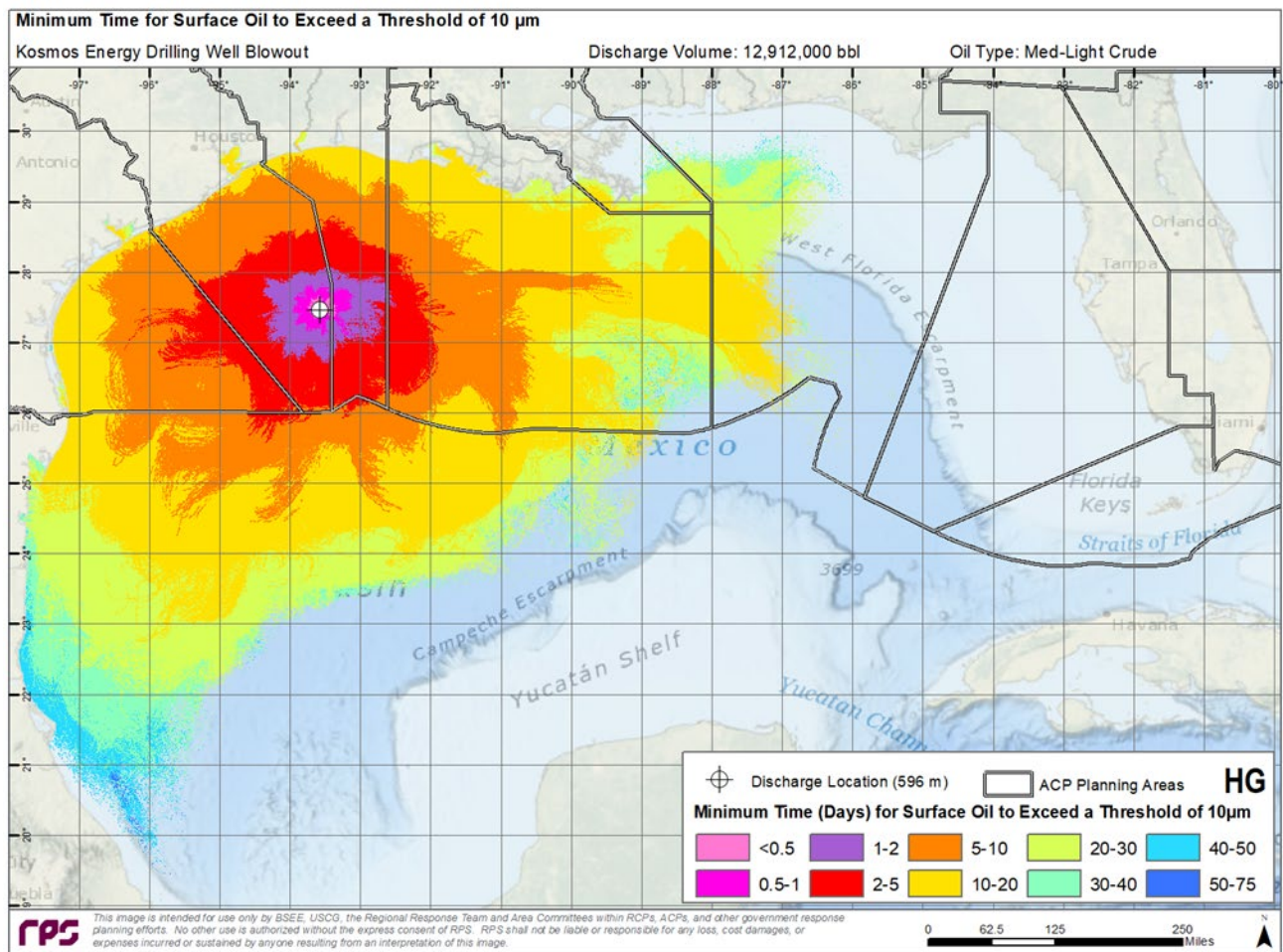
Figure 11. Minimum Travel Time for Oil on the Water Surface with Average Thickness greater than the Ecological Threshold of 10 µm.
