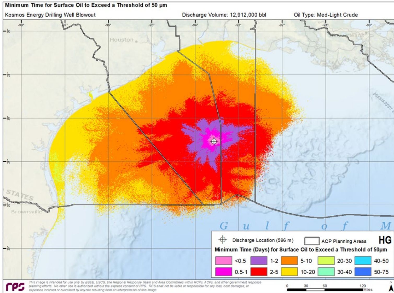
Figure 17. Minimum Travel Time for Surface Oil exposure greater than 50 \mu m.
