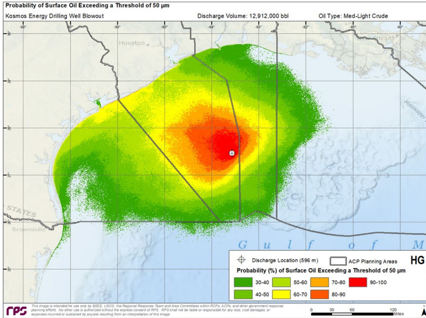
Figure 16. Probability Footprint for Surface Oil exposure greater than 50 \mu m. In this thickness range, oil will appear as a continuous to discontinuous patches of dark oil in quantities where high volume on-water mechanical recovery operations will be the most productive.
